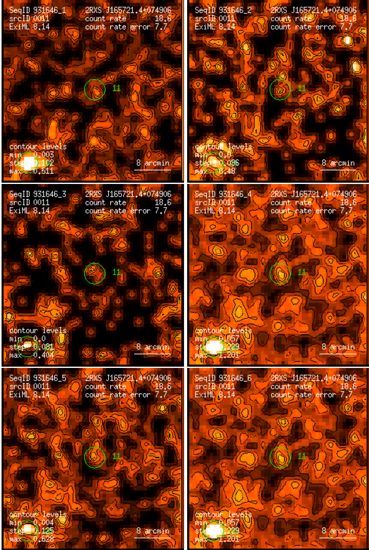
Figure 11: RASS 931646: detection 0011: band rate images, Gaussian filter: (1) PSPC channels 11 – 41, (2) 52 – 90, (3) 91 – 201, (4) 11 – 235, (5) 52 – 201, (6) 11 – 201. Broad band rates in counts/ks. Band rate contour levels in counts/ks/arcmin 2 .
