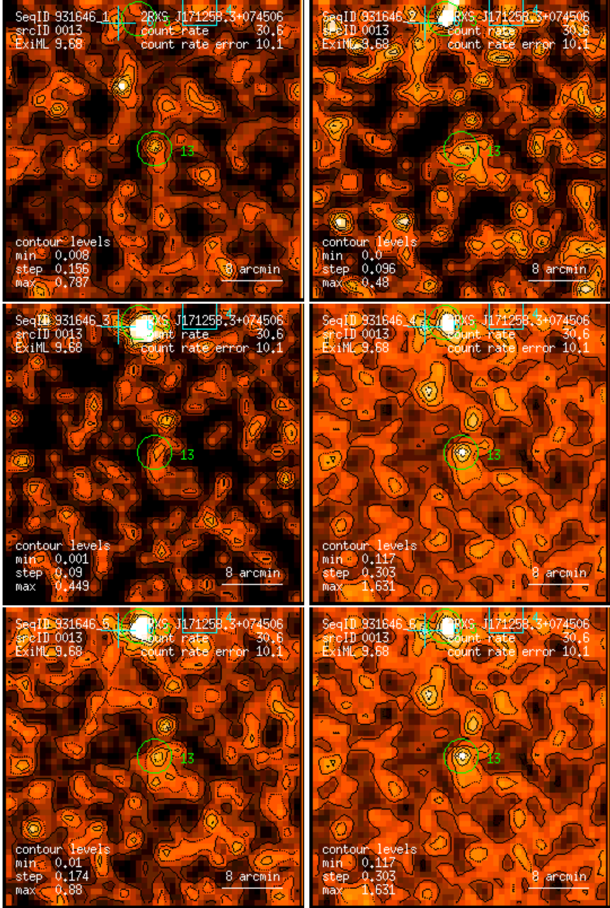
Figure 13: RASS 931646: detection 0013: band rate images, Gaussian filter: (1) PSPC channels 11 – 41, (2) 52 – 90, (3) 91 – 201, (4) 11 – 235, (5) 52 – 201, (6) 11 – 201. Broad band rates in counts/ks. Band rate contour levels in counts/ks/arcmin 2 .
