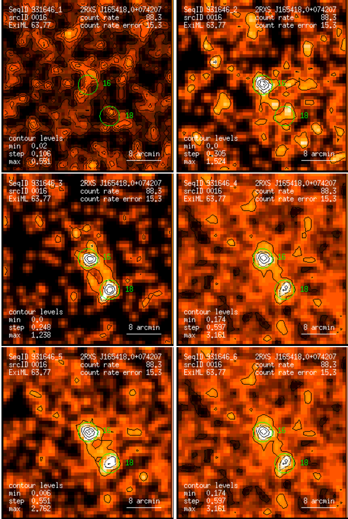
Figure 16: RASS 931646: detection 0016: band rate images, Gaussian filter: (1) PSPC channels 11 – 41, (2) 52 – 90, (3) 91 – 201, (4) 11 – 235, (5) 52 – 201, (6) 11 – 201. Broad band rates in counts/ks. Band rate contour levels in counts/ks/arcmin 2 .
