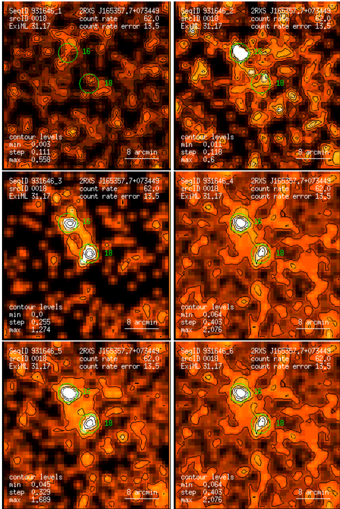
Figure 18: RASS 931646: detection 0018: band rate images, Gaussian filter: (1) PSPC channels 11 – 41, (2) 52 – 90, (3) 91 – 201, (4) 11 – 235, (5) 52 – 201, (6) 11 – 201. Broad band rates in counts/ks. Band rate contour levels in counts/ks/arcmin 2 .
