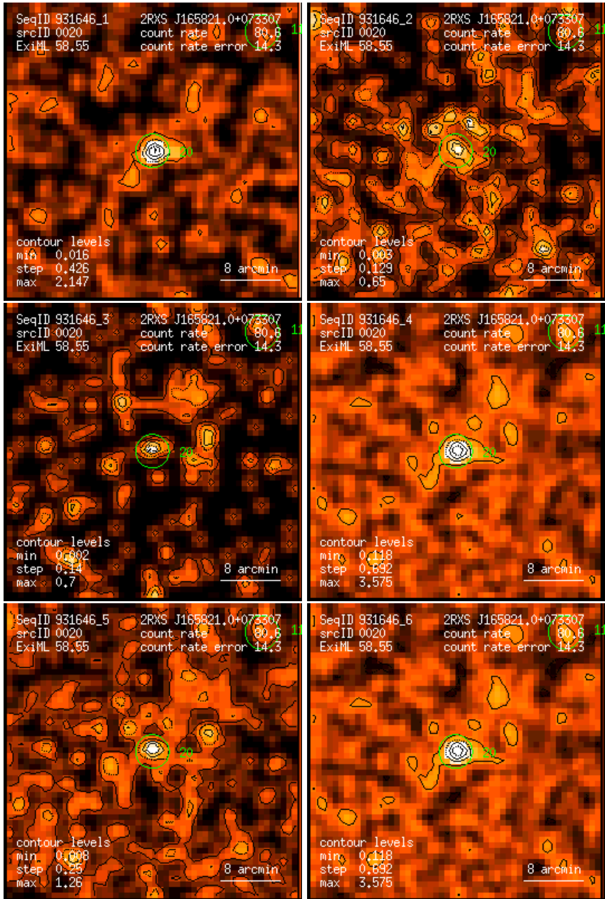
Figure 20: RASS 931646: detection 0020: band rate images, Gaussian filter: (1) PSPC channels 11 – 41, (2) 52 – 90, (3) 91 – 201, (4) 11 – 235, (5) 52 – 201, (6) 11 – 201. Broad band rates in counts/ks. Band rate contour levels in counts/ks/arcmin 2 .
