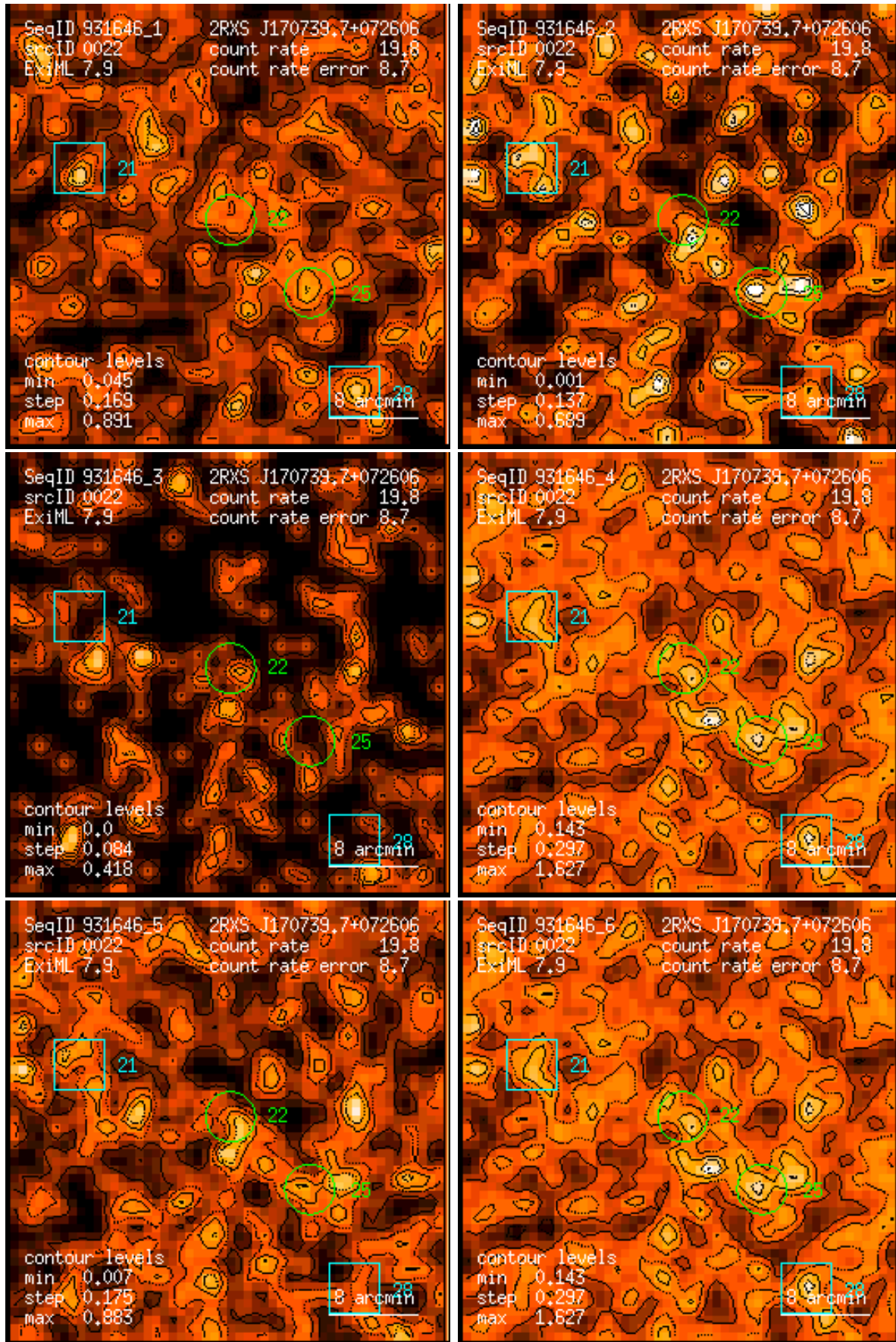
Figure 22: RASS 931646: detection 0022: band rate images, Gaussian filter: (1) PSPC channels 11 – 41, (2) 52 – 90, (3) 91 – 201, (4) 11 – 235, (5) 52 – 201, (6) 11 – 201. Broad band rates in counts/ks. Band rate contour levels in counts/ks/arcmin 2 .
