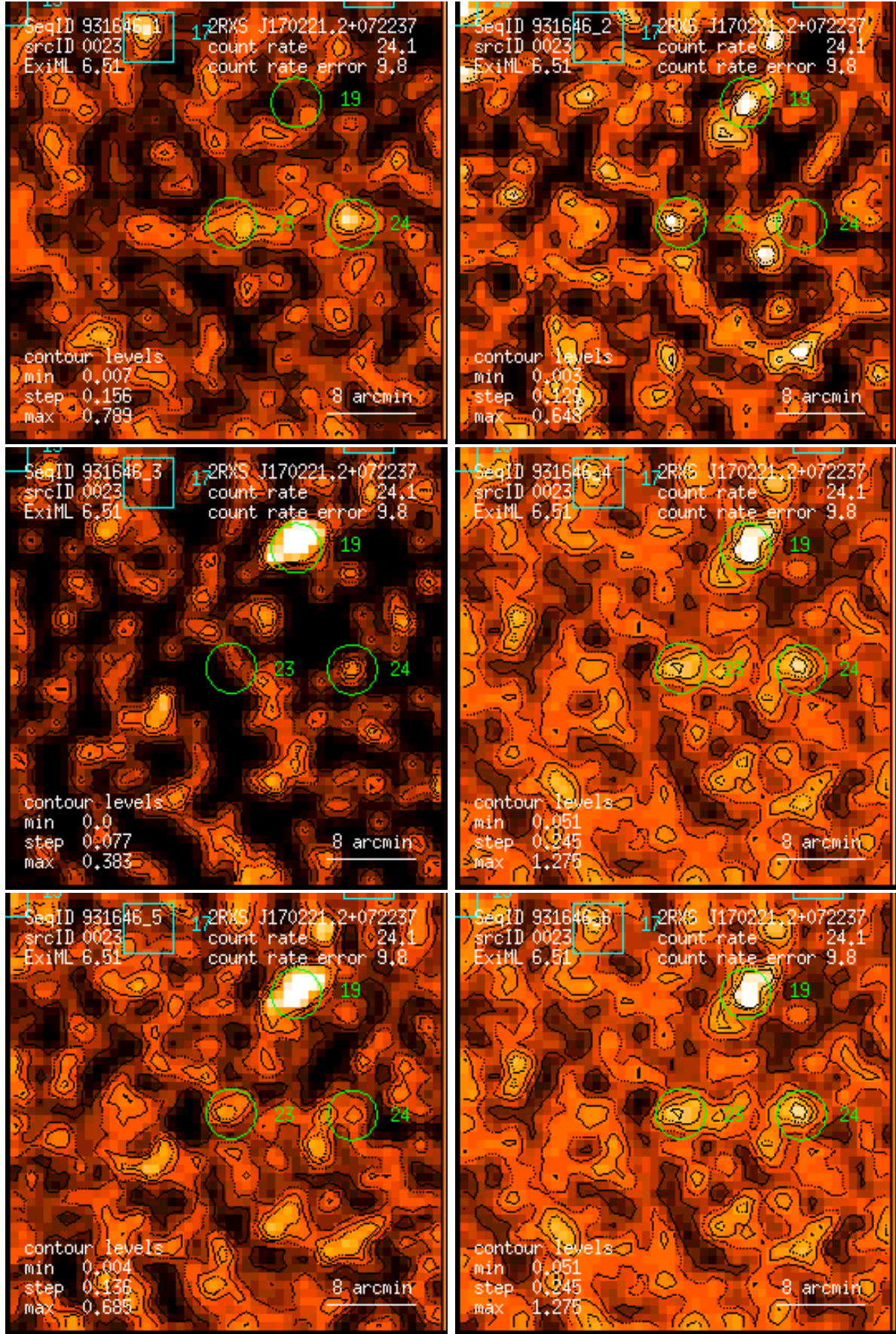
Figure 23: RASS 931646: detection 0023: band rate images, Gaussian filter: (1) PSPC channels 11 – 41, (2) 52 – 90, (3) 91 – 201, (4) 11 – 235, (5) 52 – 201, (6) 11 – 201. Broad band rates in counts/ks. Band rate contour levels in counts/ks/arcmin 2 .
