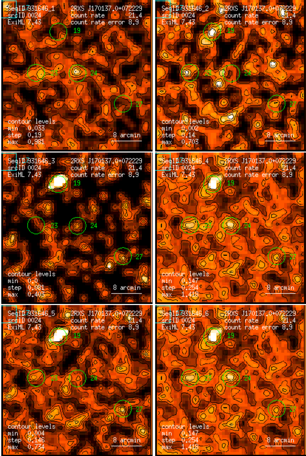
Figure 24: RASS 931646: detection 0024: band rate images, Gaussian filter: (1) PSPC channels 11 – 41, (2) 52 – 90, (3) 91 – 201, (4) 11 – 235, (5) 52 – 201, (6) 11 – 201. Broad band rates in counts/ks. Band rate contour levels in counts/ks/arcmin 2 .
