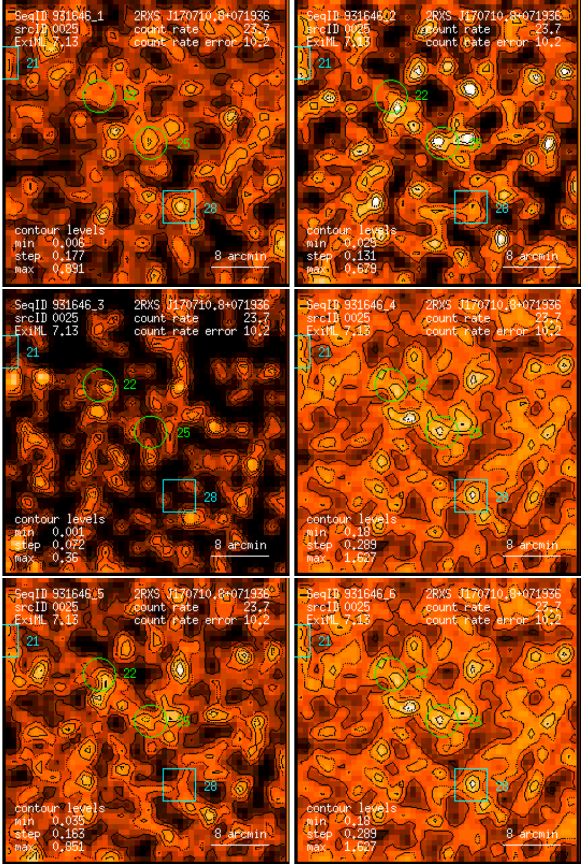
Figure 25: RASS 931646: detection 0025: band rate images, Gaussian filter: (1) PSPC channels 11 – 41, (2) 52 – 90, (3) 91 – 201, (4) 11 – 235, (5) 52 – 201, (6) 11 – 201. Broad band rates in counts/ks. Band rate contour levels in counts/ks/arcmin 2 .
