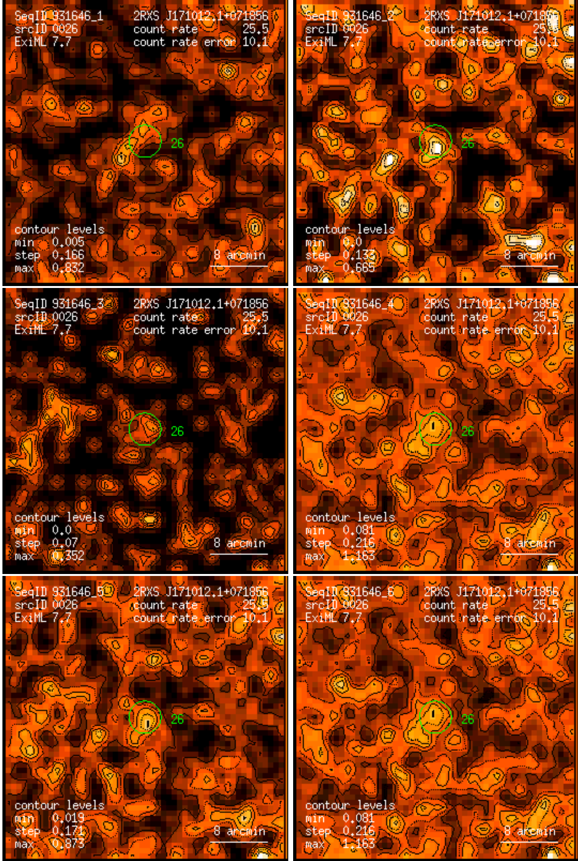
Figure 26: RASS 931646: detection 0026: band rate images, Gaussian filter: (1) PSPC channels 11 – 41, (2) 52 – 90, (3) 91 – 201, (4) 11 – 235, (5) 52 – 201, (6) 11 – 201. Broad band rates in counts/ks. Band rate contour levels in counts/ks/arcmin 2 .
