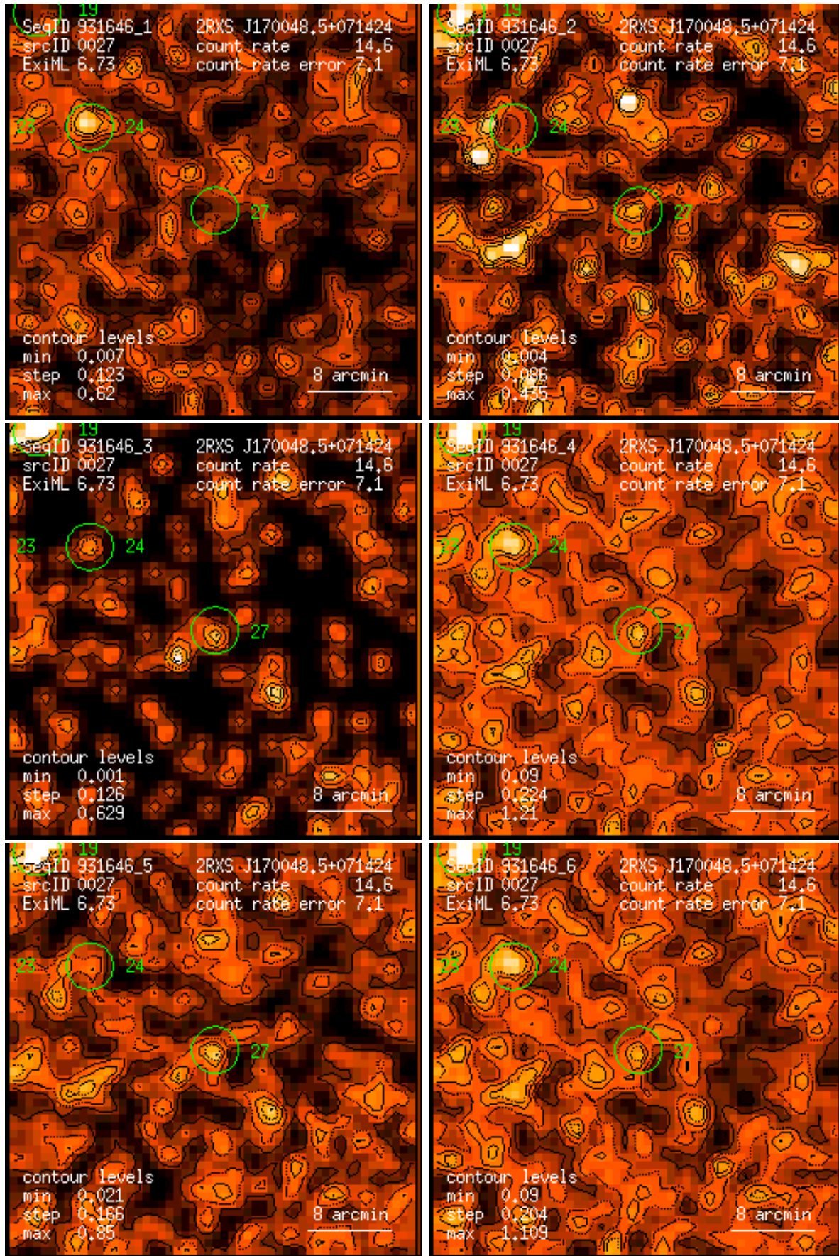
Figure 27: RASS 931646: detection 0027: band rate images, Gaussian filter: (1) PSPC channels 11 – 41, (2) 52 – 90, (3) 91 – 201, (4) 11 – 235, (5) 52 – 201, (6) 11 – 201. Broad band rates in counts/ks. Band rate contour levels in counts/ks/arcmin 2 .
