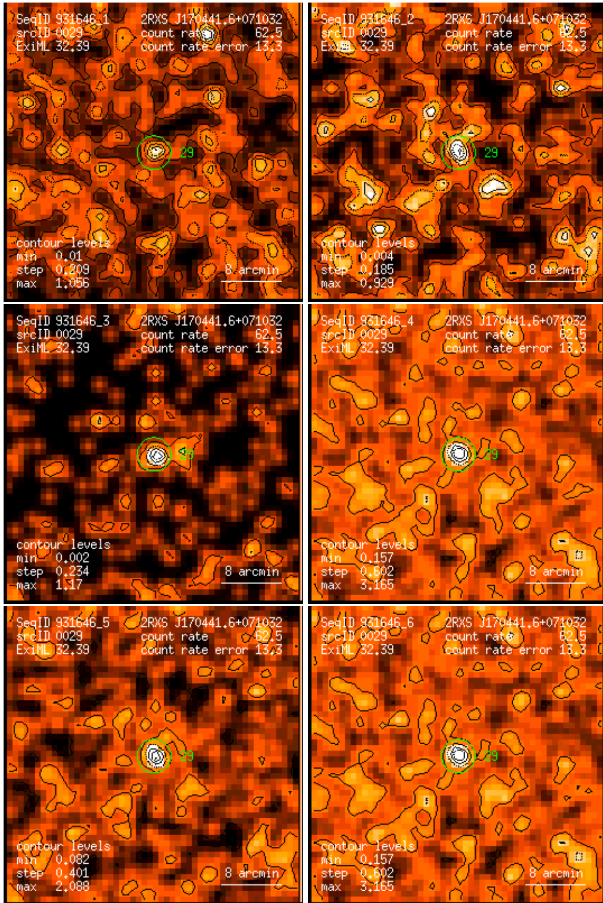
Figure 29: RASS 931646: detection 0029: band rate images, Gaussian filter: (1) PSPC channels 11 – 41, (2) 52 – 90, (3) 91 – 201, (4) 11 – 235, (5) 52 – 201, (6) 11 – 201. Broad band rates in counts/ks. Band rate contour levels in counts/ks/arcmin 2 .
