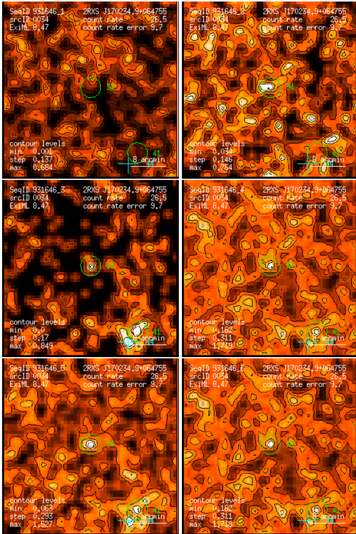
Figure 34: RASS 931646: detection 0034: band rate images, Gaussian filter: (1) PSPC channels 11 – 41, (2) 52 – 90, (3) 91 – 201, (4) 11 – 235, (5) 52 – 201, (6) 11 – 201. Broad band rates in counts/ks. Band rate contour levels in counts/ks/arcmin 2 .
