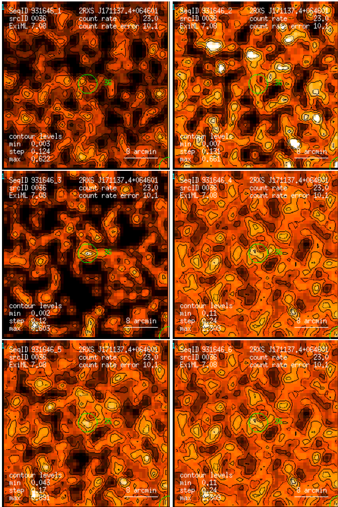
Figure 36: RASS 931646: detection 0036: band rate images, Gaussian filter: (1) PSPC channels 11 – 41, (2) 52 – 90, (3) 91 – 201, (4) 11 – 235, (5) 52 – 201, (6) 11 – 201. Broad band rates in counts/ks. Band rate contour levels in counts/ks/arcmin 2 .
