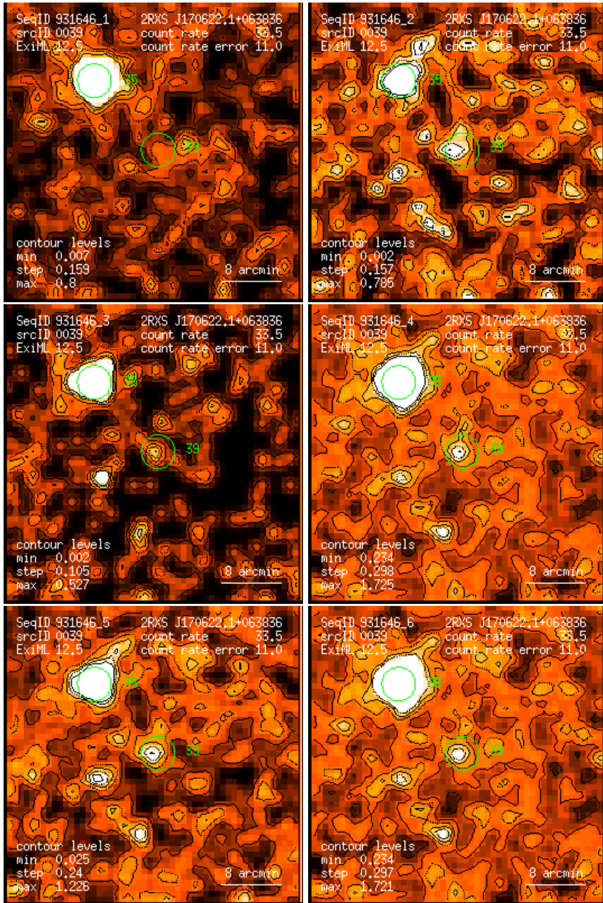
Figure 39: RASS 931646: detection 0039: band rate images, Gaussian filter: (1) PSPC channels 11 – 41, (2) 52 – 90, (3) 91 – 201, (4) 11 – 235, (5) 52 – 201, (6) 11 – 201. Broad band rates in counts/ks. Band rate contour levels in counts/ks/arcmin 2 .
