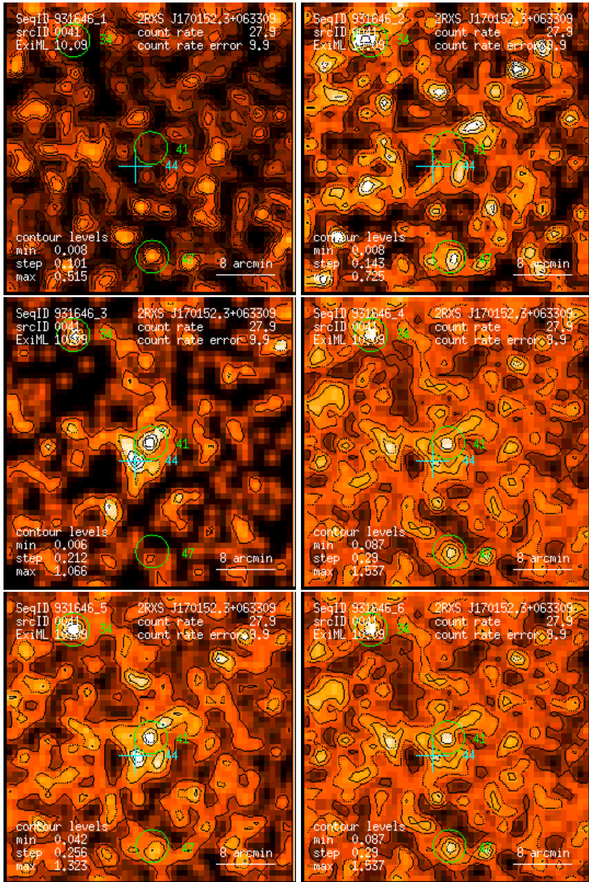
Figure 41: RASS 931646: detection 0041: band rate images, Gaussian filter: (1) PSPC channels 11 – 41, (2) 52 – 90, (3) 91 – 201, (4) 11 – 235, (5) 52 – 201, (6) 11 – 201. Broad band rates in counts/ks. Band rate contour levels in counts/ks/arcmin 2 .
