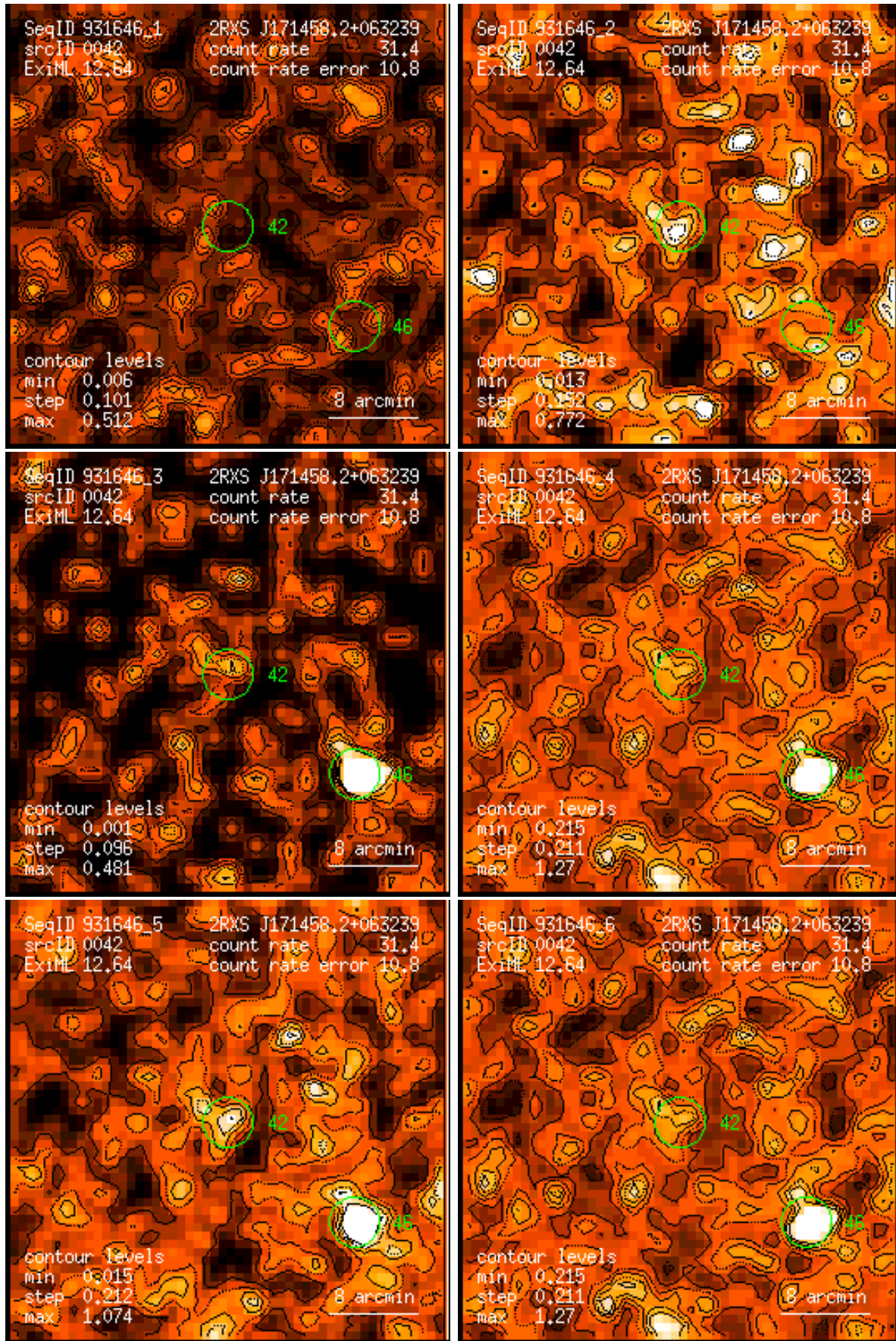
Figure 42: RASS 931646: detection 0042: band rate images, Gaussian filter: (1) PSPC channels 11 – 41, (2) 52 – 90, (3) 91 – 201, (4) 11 – 235, (5) 52 – 201, (6) 11 – 201. Broad band rates in counts/ks. Band rate contour levels in counts/ks/arcmin 2 .
