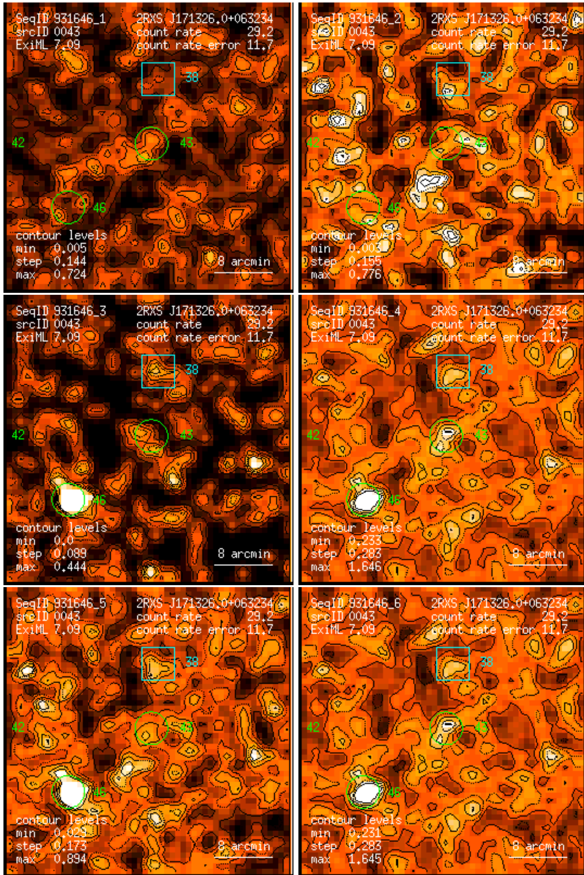
Figure 43: RASS 931646: detection 0043: band rate images, Gaussian filter: (1) PSPC channels 11 – 41, (2) 52 – 90, (3) 91 – 201, (4) 11 – 235, (5) 52 – 201, (6) 11 – 201. Broad band rates in counts/ks. Band rate contour levels in counts/ks/arcmin 2 .
