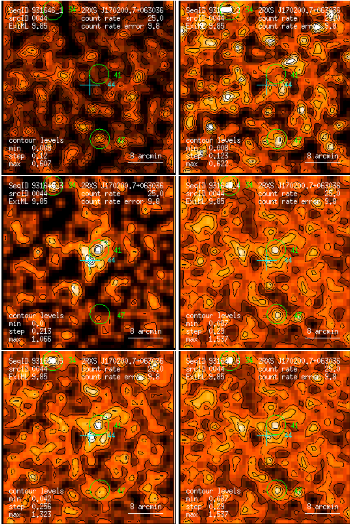
Figure 44: RASS 931646: detection 0044: band rate images, Gaussian filter: (1) PSPC channels 11 – 41, (2) 52 – 90, (3) 91 – 201, (4) 11 – 235, (5) 52 – 201, (6) 11 – 201. Broad band rates in counts/ks. Band rate contour levels in counts/ks/arcmin 2 .
