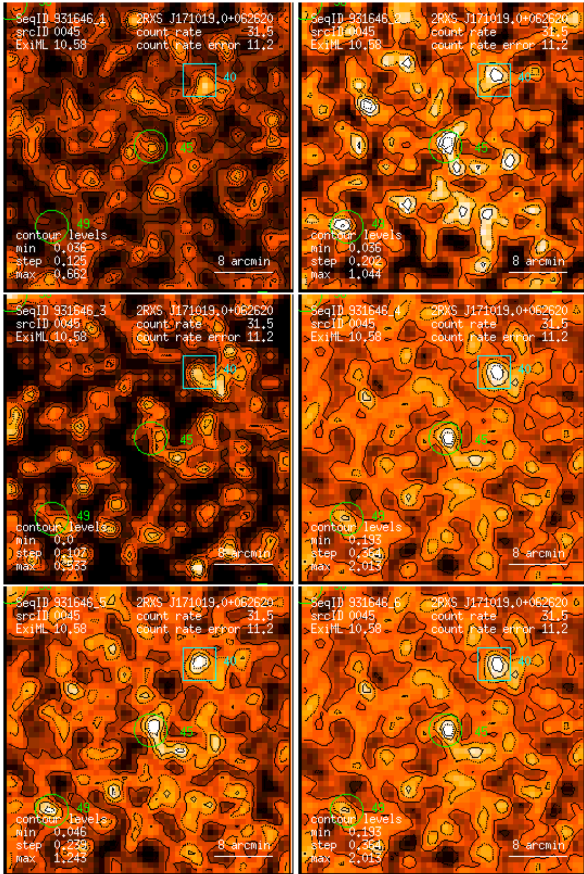
Figure 45: RASS 931646: detection 0045: band rate images, Gaussian filter: (1) PSPC channels 11 – 41, (2) 52 – 90, (3) 91 – 201, (4) 11 – 235, (5) 52 – 201, (6) 11 – 201. Broad band rates in counts/ks. Band rate contour levels in counts/ks/arcmin 2 .
