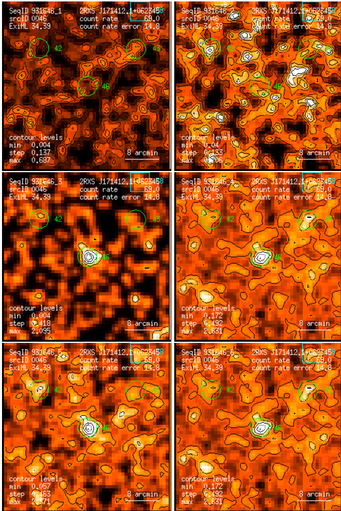
Figure 46: RASS 931646: detection 0046: band rate images, Gaussian filter: (1) PSPC channels 11 – 41, (2) 52 – 90, (3) 91 – 201, (4) 11 – 235, (5) 52 – 201, (6) 11 – 201. Broad band rates in counts/ks. Band rate contour levels in counts/ks/arcmin 2 .
