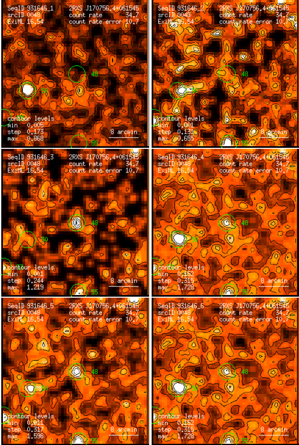
Figure 48: RASS 931646: detection 0048: band rate images, Gaussian filter: (1) PSPC channels 11 – 41, (2) 52 – 90, (3) 91 – 201, (4) 11 – 235, (5) 52 – 201, (6) 11 – 201. Broad band rates in counts/ks. Band rate contour levels in counts/ks/arcmin 2 .
