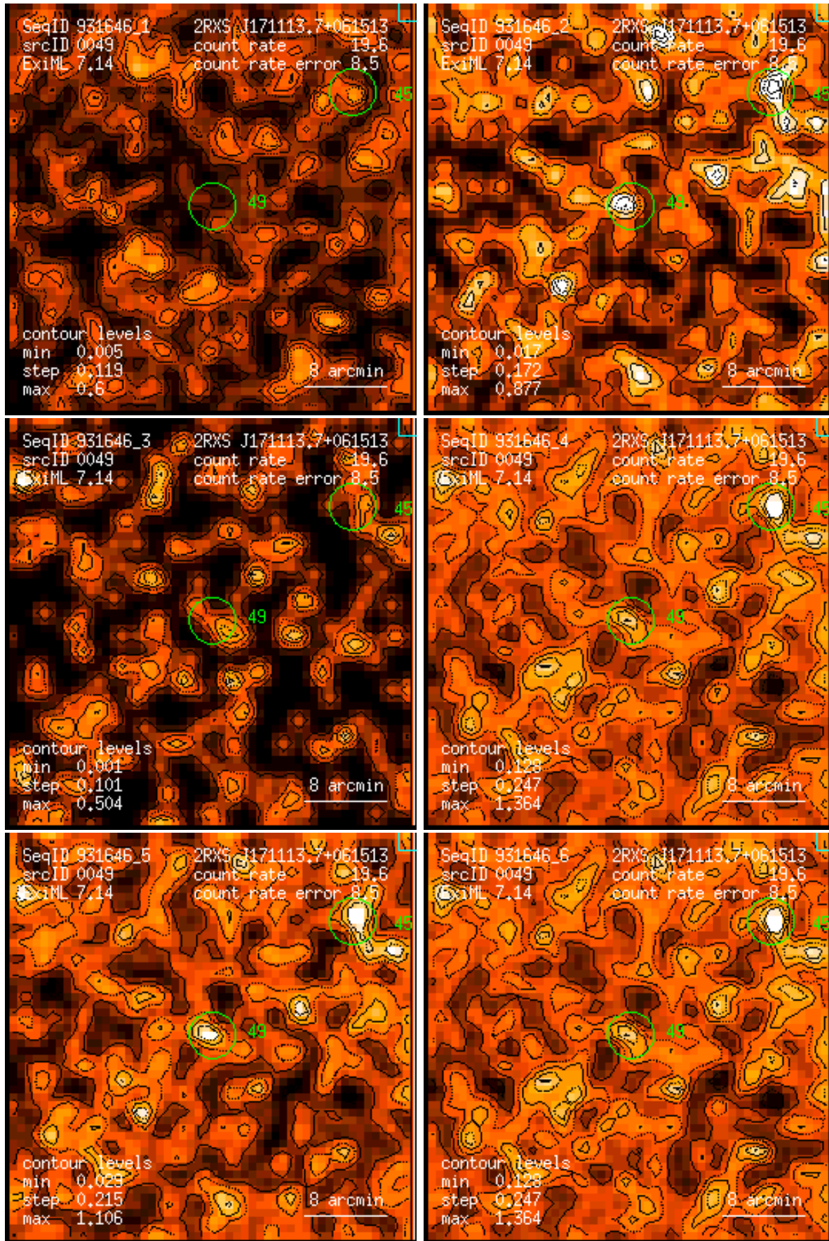
Figure 49: RASS 931646: detection 0049: band rate images, Gaussian filter: (1) PSPC channels 11 – 41, (2) 52 – 90, (3) 91 – 201, (4) 11 – 235, (5) 52 – 201, (6) 11 – 201. Broad band rates in counts/ks. Band rate contour levels in counts/ks/arcmin 2 .
