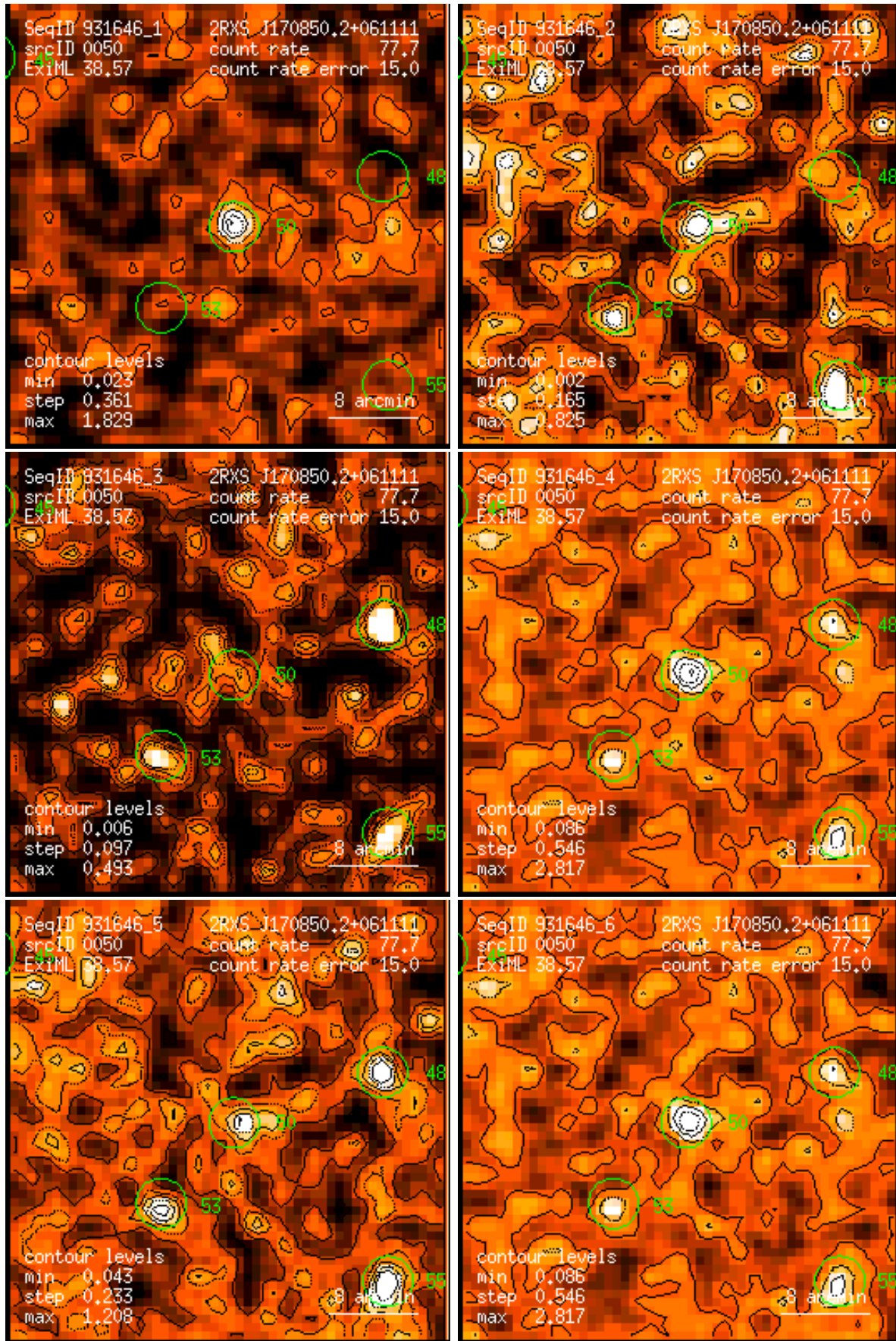
Figure 50: RASS 931646: detection 0050: band rate images, Gaussian filter: (1) PSPC channels 11 – 41, (2) 52 – 90, (3) 91 – 201, (4) 11 – 235, (5) 52 – 201, (6) 11 – 201. Broad band rates in counts/ks. Band rate contour levels in counts/ks/arcmin 2 .
