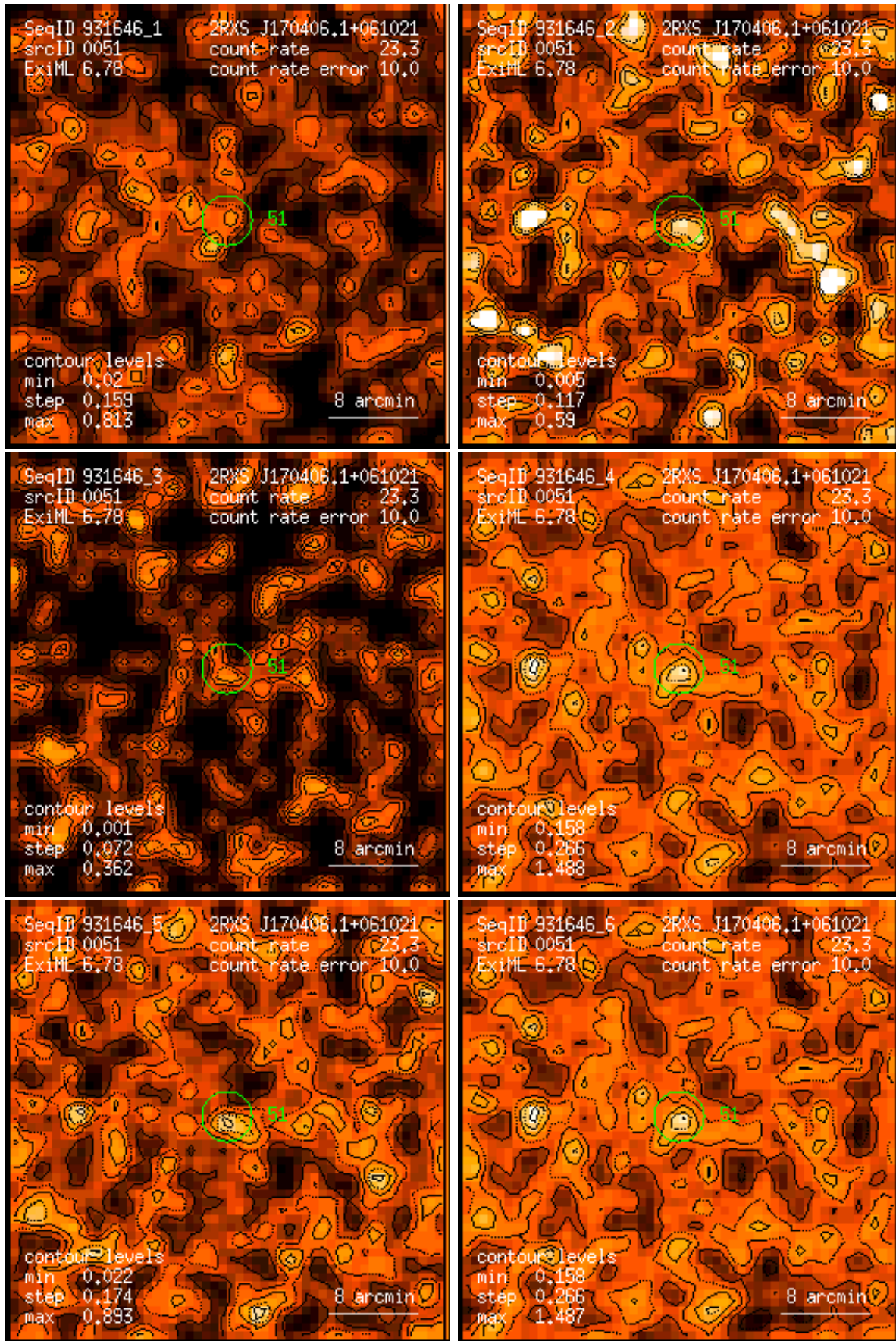
Figure 51: RASS 931646: detection 0051: band rate images, Gaussian filter: (1) PSPC channels 11 – 41, (2) 52 – 90, (3) 91 – 201, (4) 11 – 235, (5) 52 – 201, (6) 11 – 201. Broad band rates in counts/ks. Band rate contour levels in counts/ks/arcmin 2 .
