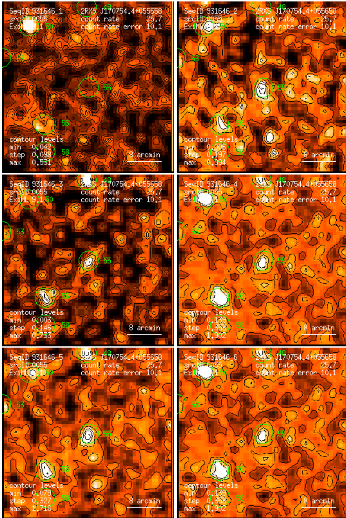
Figure 55: RASS 931646: detection 0055: band rate images, Gaussian filter: (1) PSPC channels 11 – 41, (2) 52 – 90, (3) 91 – 201, (4) 11 – 235, (5) 52 – 201, (6) 11 – 201. Broad band rates in counts/ks. Band rate contour levels in counts/ks/arcmin 2 .
