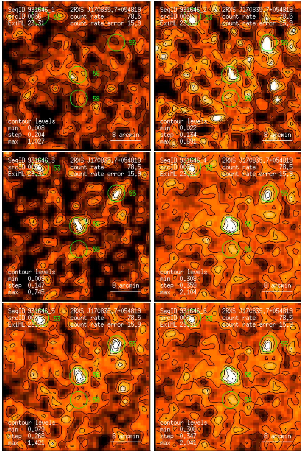
Figure 56: RASS 931646: detection 0056: band rate images, Gaussian filter: (1) PSPC channels 11 – 41, (2) 52 – 90, (3) 91 – 201, (4) 11 – 235, (5) 52 – 201, (6) 11 – 201. Broad band rates in counts/ks. Band rate contour levels in counts/ks/arcmin 2 .
