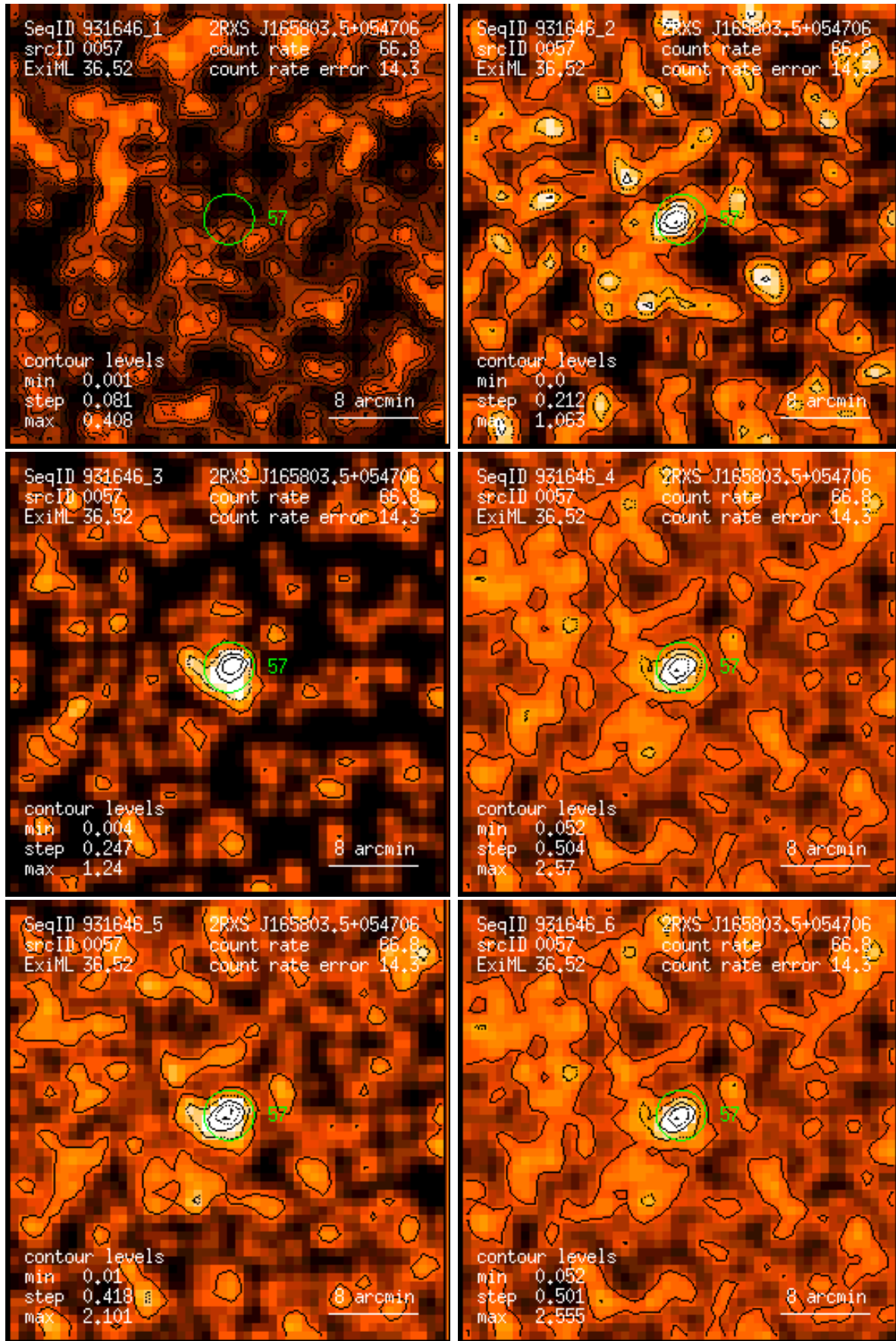
Figure 57: RASS 931646: detection 0057: band rate images, Gaussian filter: (1) PSPC channels 11 – 41, (2) 52 – 90, (3) 91 – 201, (4) 11 – 235, (5) 52 – 201, (6) 11 – 201. Broad band rates in counts/ks. Band rate contour levels in counts/ks/arcmin 2 .
