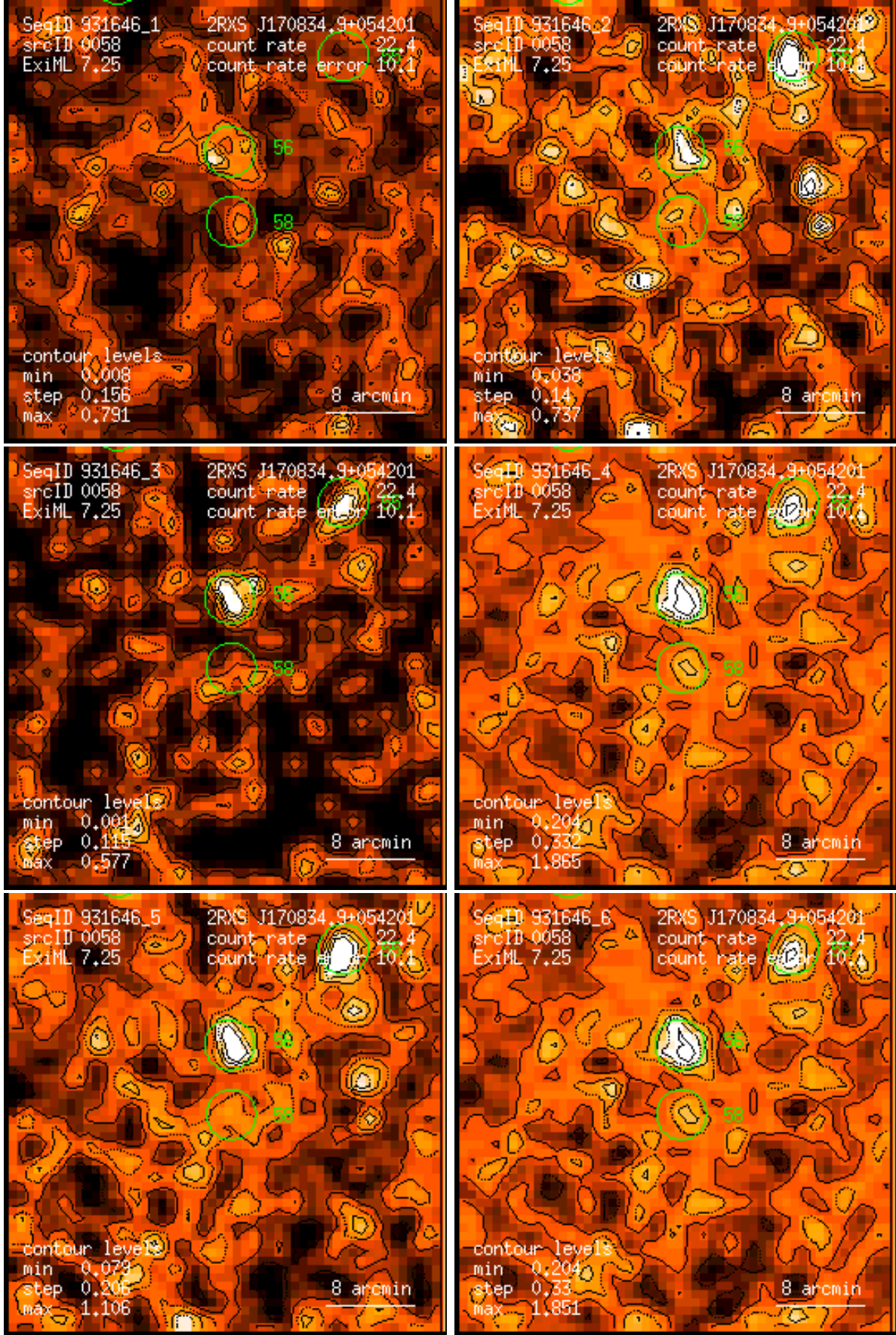
Figure 58: RASS 931646: detection 0058: band rate images, Gaussian filter: (1) PSPC channels 11 – 41, (2) 52 – 90, (3) 91 – 201, (4) 11 – 235, (5) 52 – 201, (6) 11 – 201. Broad band rates in counts/ks. Band rate contour levels in counts/ks/arcmin 2 .
