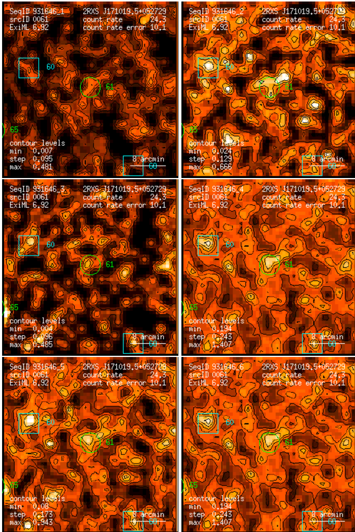
Figure 61: RASS 931646: detection 0061: band rate images, Gaussian filter: (1) PSPC channels 11 – 41, (2) 52 – 90, (3) 91 – 201, (4) 11 – 235, (5) 52 – 201, (6) 11 – 201. Broad band rates in counts/ks. Band rate contour levels in counts/ks/arcmin 2 .
