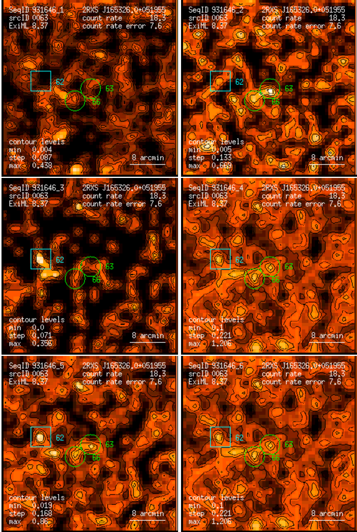
Figure 63: RASS 931646: detection 0063: band rate images, Gaussian filter: (1) PSPC channels 11 – 41, (2) 52 – 90, (3) 91 – 201, (4) 11 – 235, (5) 52 – 201, (6) 11 – 201. Broad band rates in counts/ks. Band rate contour levels in counts/ks/arcmin 2 .
