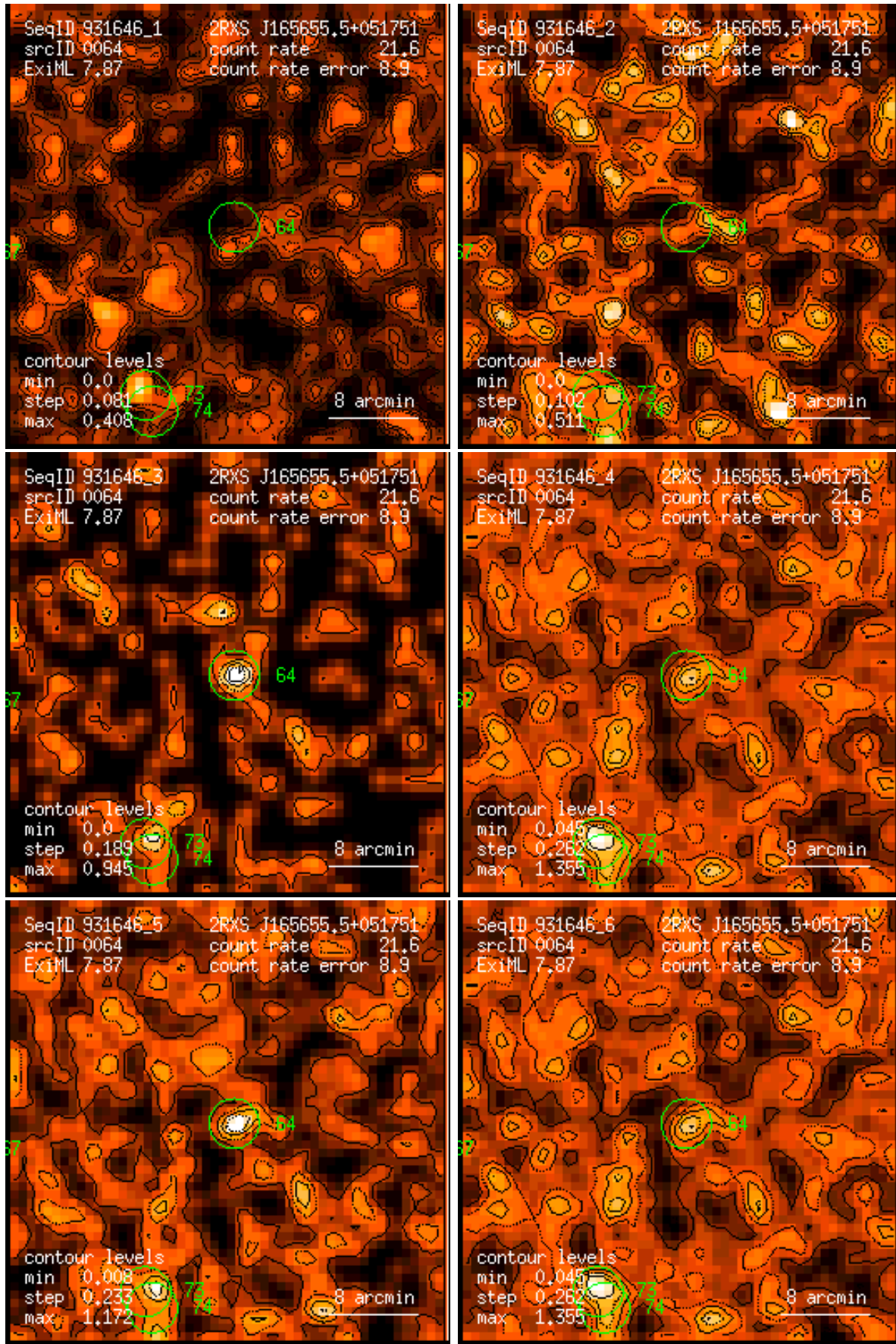
Figure 64: RASS 931646: detection 0064: band rate images, Gaussian filter: (1) PSPC channels 11 – 41, (2) 52 – 90, (3) 91 – 201, (4) 11 – 235, (5) 52 – 201, (6) 11 – 201. Broad band rates in counts/ks. Band rate contour levels in counts/ks/arcmin 2 .
