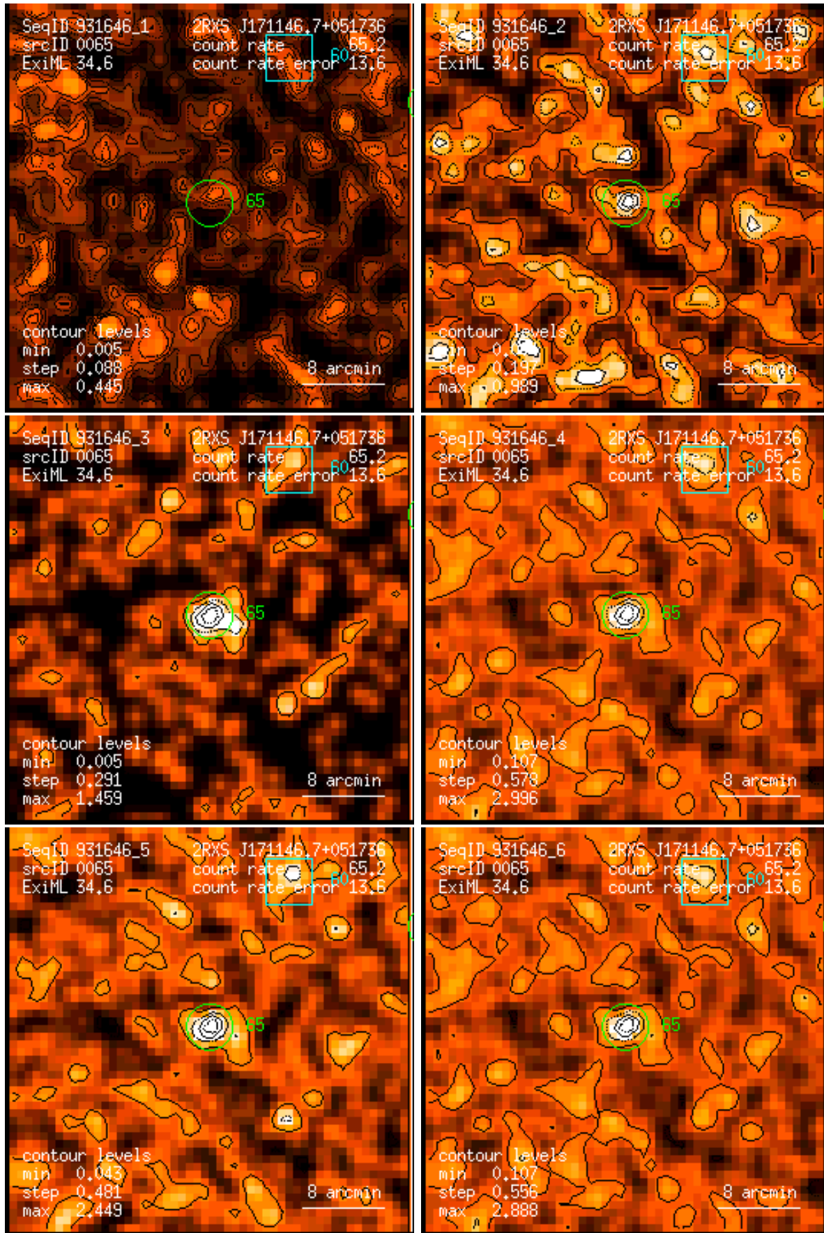
Figure 65: RASS 931646: detection 0065: band rate images, Gaussian filter: (1) PSPC channels 11 – 41, (2) 52 – 90, (3) 91 – 201, (4) 11 – 235, (5) 52 – 201, (6) 11 – 201. Broad band rates in counts/ks. Band rate contour levels in counts/ks/arcmin 2 .
