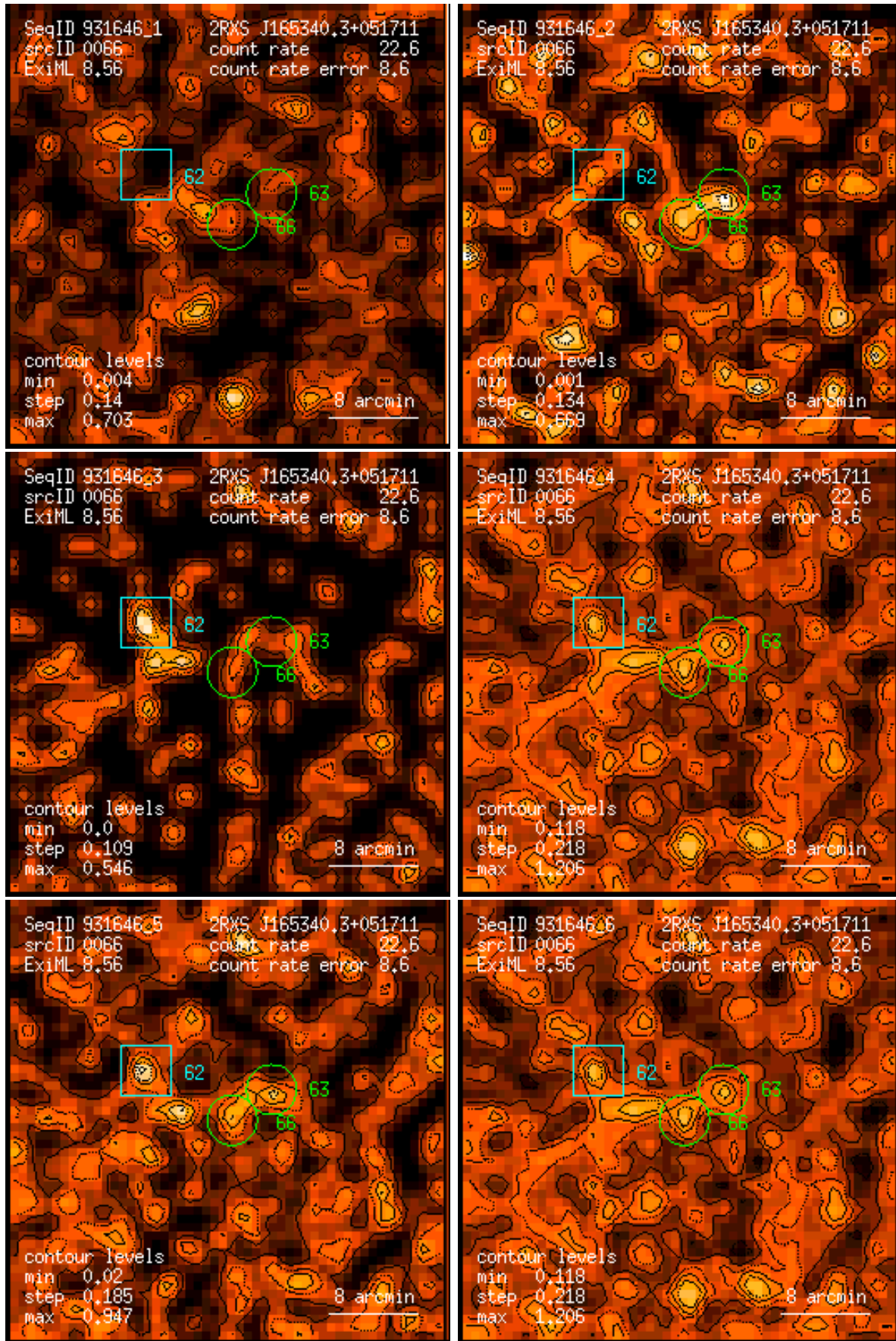
Figure 66: RASS 931646: detection 0066: band rate images, Gaussian filter: (1) PSPC channels 11 – 41, (2) 52 – 90, (3) 91 – 201, (4) 11 – 235, (5) 52 – 201, (6) 11 – 201. Broad band rates in counts/ks. Band rate contour levels in counts/ks/arcmin 2 .
