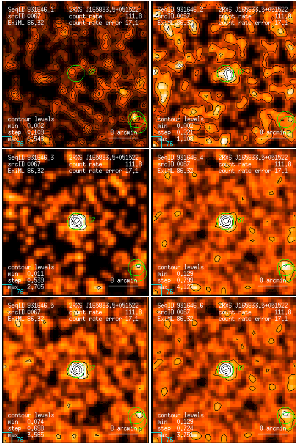
Figure 67: RASS 931646: detection 0067: band rate images, Gaussian filter: (1) PSPC channels 11 – 41, (2) 52 – 90, (3) 91 – 201, (4) 11 – 235, (5) 52 – 201, (6) 11 – 201. Broad band rates in counts/ks. Band rate contour levels in counts/ks/arcmin 2 .
