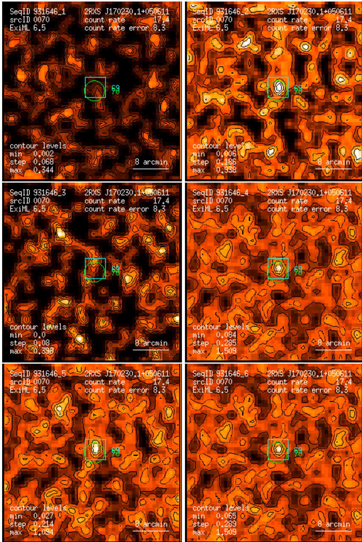
Figure 70: RASS 931646: detection 0070: band rate images, Gaussian filter: (1) PSPC channels 11 – 41, (2) 52 – 90, (3) 91 – 201, (4) 11 – 235, (5) 52 – 201, (6) 11 – 201. Broad band rates in counts/ks. Band rate contour levels in counts/ks/arcmin 2 .
