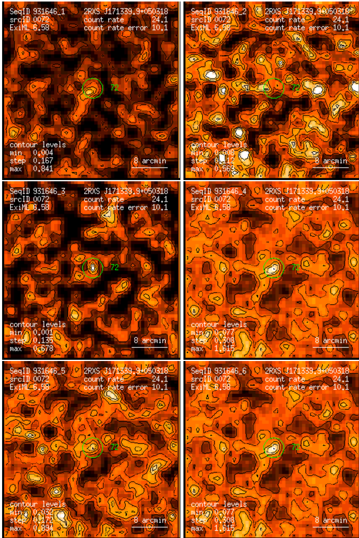
Figure 72: RASS 931646: detection 0072: band rate images, Gaussian filter: (1) PSPC channels 11 – 41, (2) 52 – 90, (3) 91 – 201, (4) 11 – 235, (5) 52 – 201, (6) 11 – 201. Broad band rates in counts/ks. Band rate contour levels in counts/ks/arcmin 2 .
