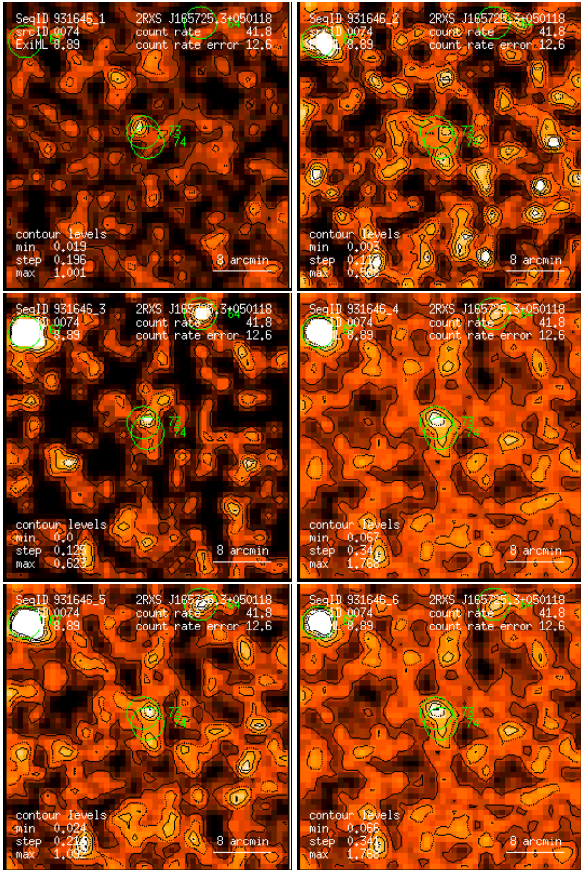
Figure 74: RASS 931646: detection 0074: band rate images, Gaussian filter: (1) PSPC channels 11 – 41, (2) 52 – 90, (3) 91 – 201, (4) 11 – 235, (5) 52 – 201, (6) 11 – 201. Broad band rates in counts/ks. Band rate contour levels in counts/ks/arcmin 2 .
