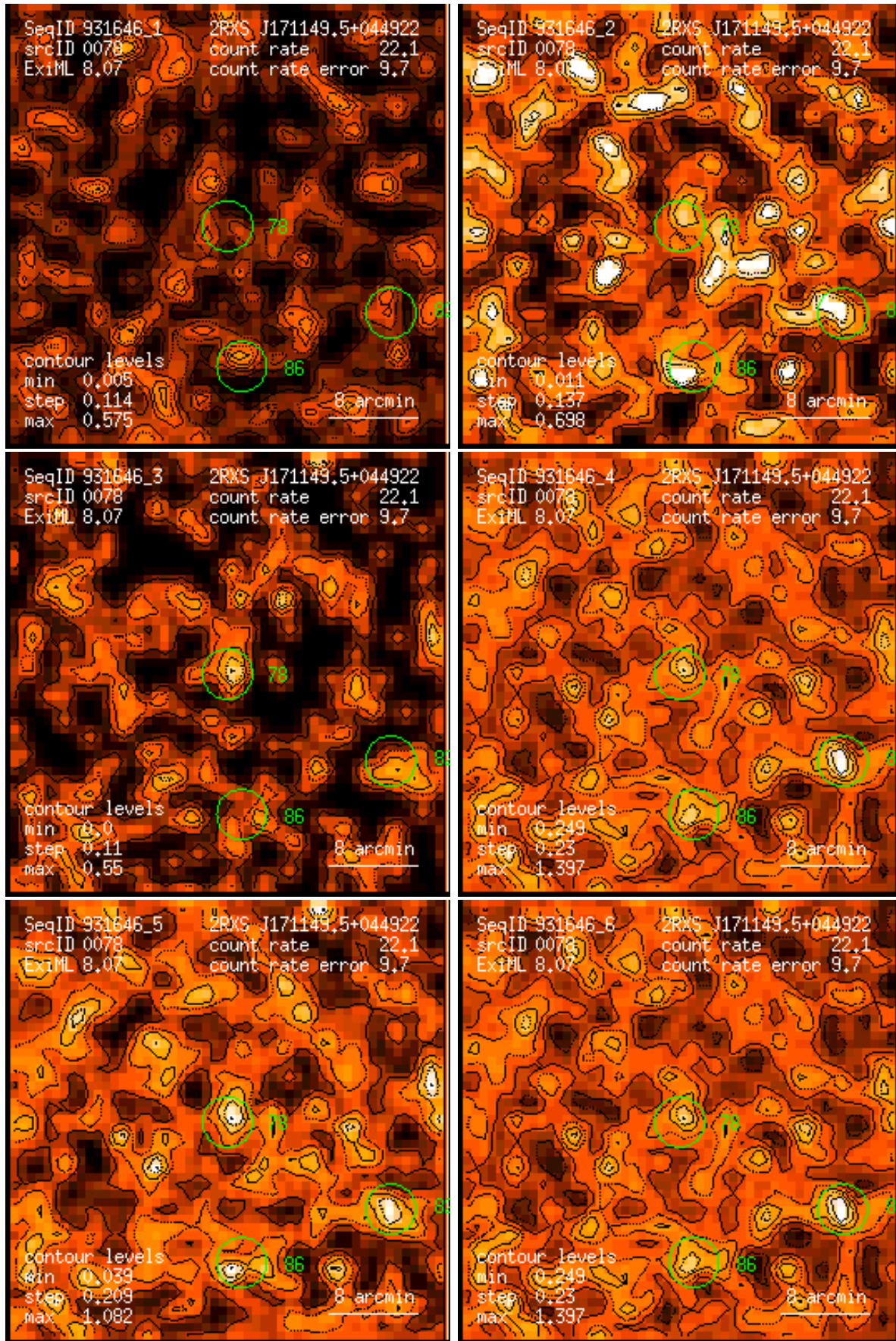
Figure 78: RASS 931646: detection 0078: band rate images, Gaussian filter: (1) PSPC channels 11 – 41, (2) 52 – 90, (3) 91 – 201, (4) 11 – 235, (5) 52 – 201, (6) 11 – 201. Broad band rates in counts/ks. Band rate contour levels in counts/ks/arcmin 2 .
