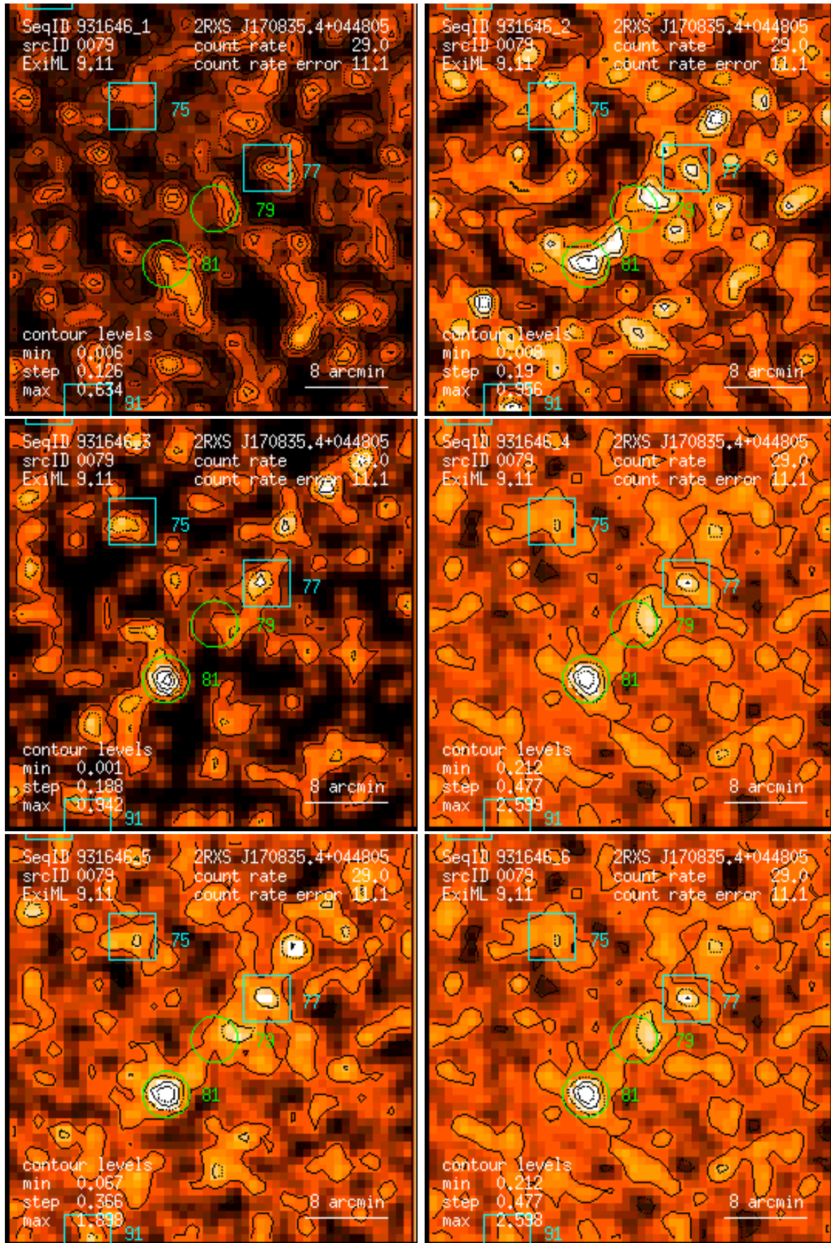
Figure 79: RASS 931646: detection 0079: band rate images, Gaussian filter: (1) PSPC channels 11 – 41, (2) 52 – 90, (3) 91 – 201, (4) 11 – 235, (5) 52 – 201, (6) 11 – 201. Broad band rates in counts/ks. Band rate contour levels in counts/ks/arcmin 2 .
