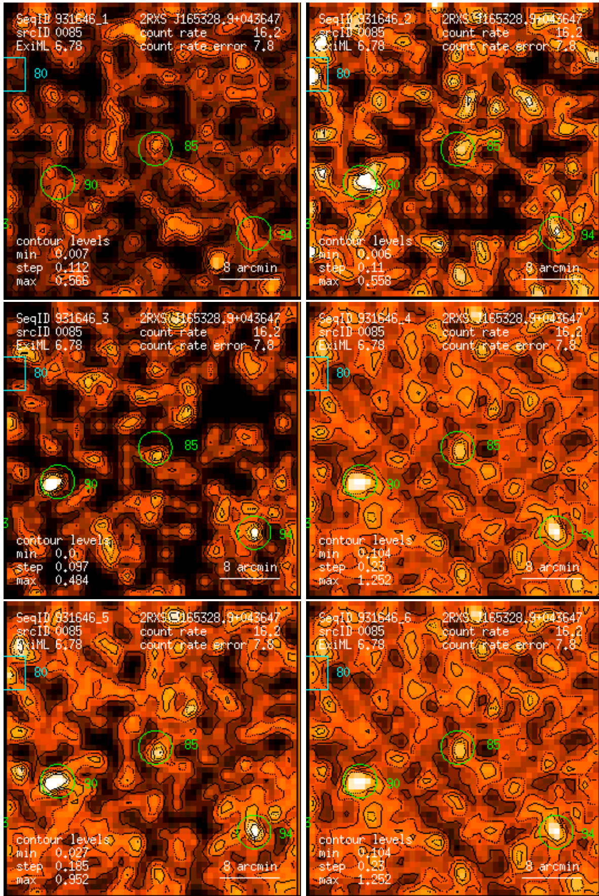
Figure 85: RASS 931646: detection 0085: band rate images, Gaussian filter: (1) PSPC channels 11 – 41, (2) 52 – 90, (3) 91 – 201, (4) 11 – 235, (5) 52 – 201, (6) 11 – 201. Broad band rates in counts/ks. Band rate contour levels in counts/ks/arcmin 2 .
