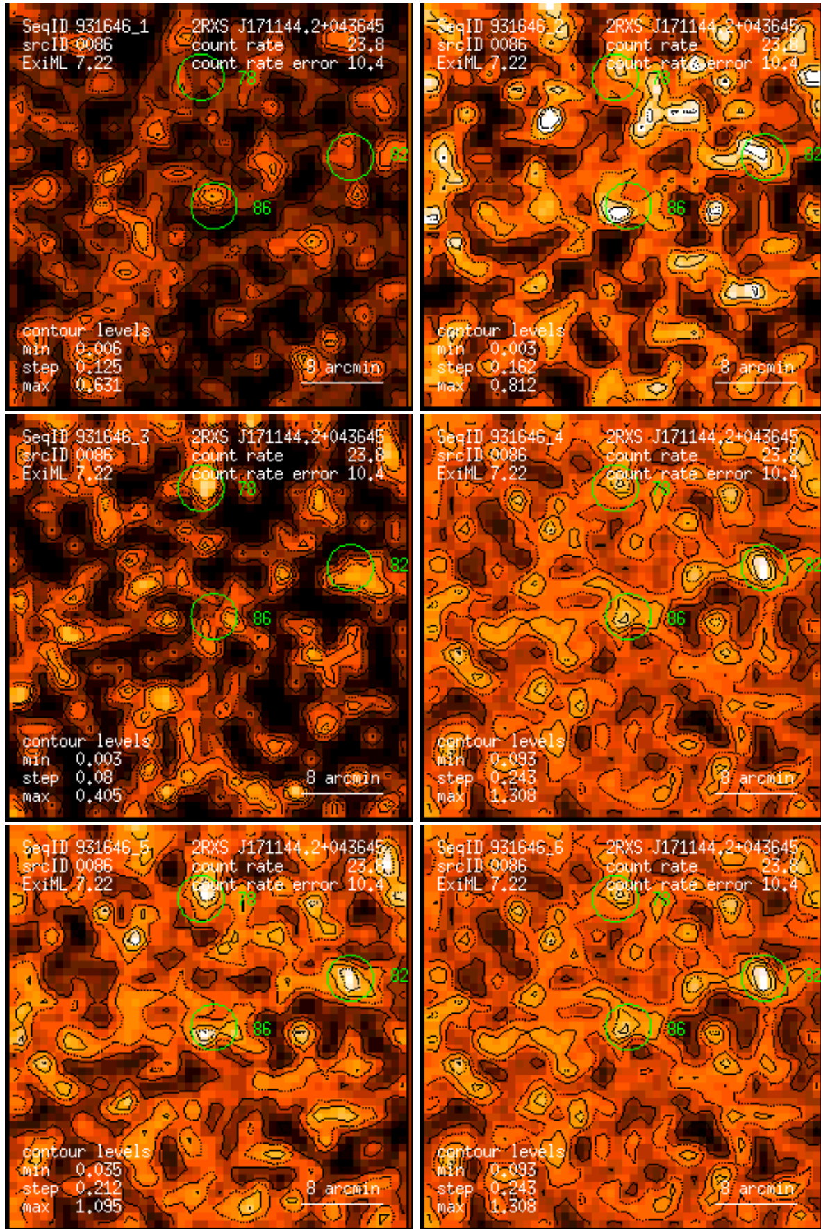
Figure 86: RASS 931646: detection 0086: band rate images, Gaussian filter: (1) PSPC channels 11 – 41, (2) 52 – 90, (3) 91 – 201, (4) 11 – 235, (5) 52 – 201, (6) 11 – 201. Broad band rates in counts/ks. Band rate contour levels in counts/ks/arcmin 2 .
