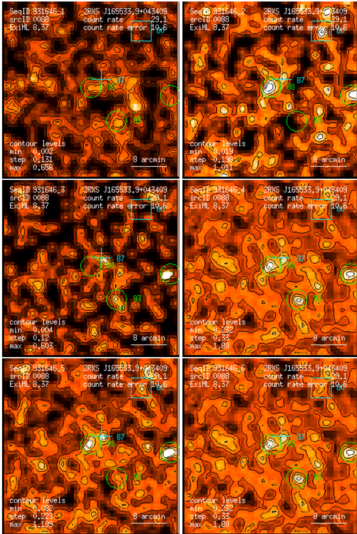
Figure 88: RASS 931646: detection 0088: band rate images, Gaussian filter: (1) PSPC channels 11 – 41, (2) 52 – 90, (3) 91 – 201, (4) 11 – 235, (5) 52 – 201, (6) 11 – 201. Broad band rates in counts/ks. Band rate contour levels in counts/ks/arcmin 2 .
