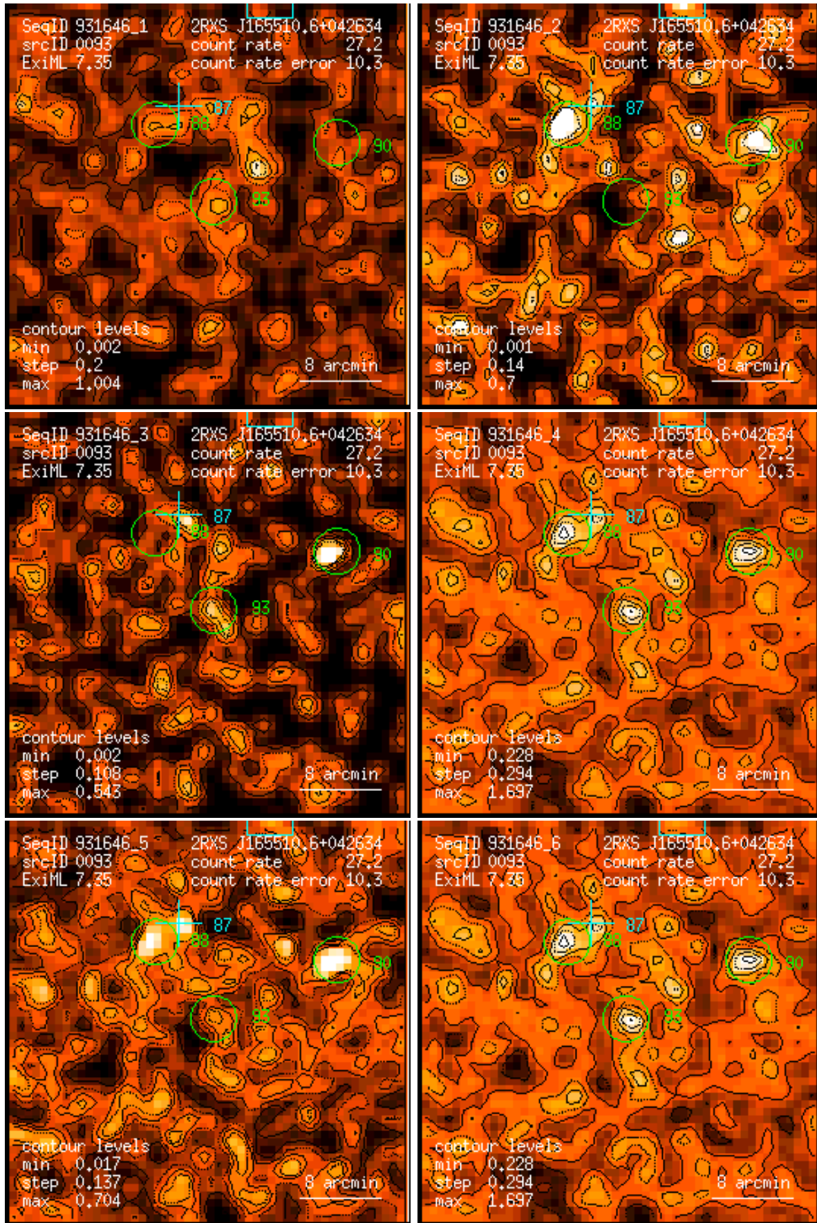
Figure 93: RASS 931646: detection 0093: band rate images, Gaussian filter: (1) PSPC channels 11 – 41, (2) 52 – 90, (3) 91 – 201, (4) 11 – 235, (5) 52 – 201, (6) 11 – 201. Broad band rates in counts/ks. Band rate contour levels in counts/ks/arcmin 2 .
