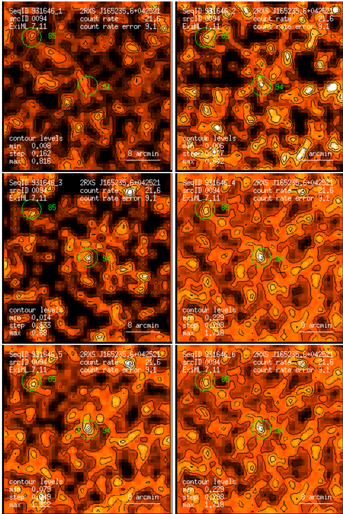
Figure 94: RASS 931646: detection 0094: band rate images, Gaussian filter: (1) PSPC channels 11 – 41, (2) 52 – 90, (3) 91 – 201, (4) 11 – 235, (5) 52 – 201, (6) 11 – 201. Broad band rates in counts/ks. Band rate contour levels in counts/ks/arcmin 2 .
