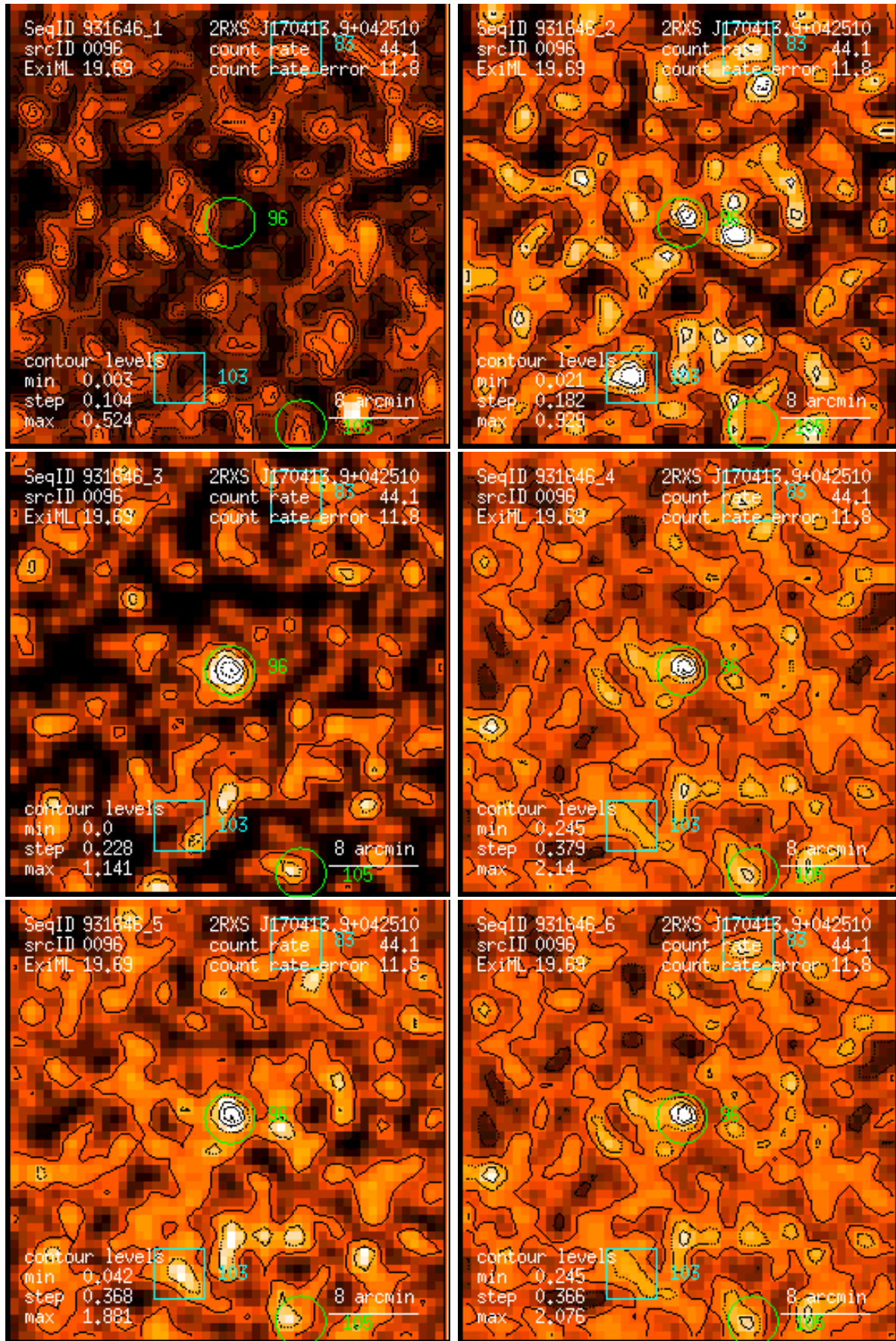
Figure 96: RASS 931646: detection 0096: band rate images, Gaussian filter: (1) PSPC channels 11 – 41, (2) 52 – 90, (3) 91 – 201, (4) 11 – 235, (5) 52 – 201, (6) 11 – 201. Broad band rates in counts/ks. Band rate contour levels in counts/ks/arcmin 2 .
