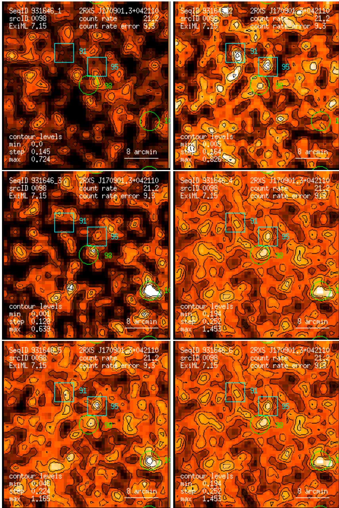
Figure 98: RASS 931646: detection 0098: band rate images, Gaussian filter: (1) PSPC channels 11 – 41, (2) 52 – 90, (3) 91 – 201, (4) 11 – 235, (5) 52 – 201, (6) 11 – 201. Broad band rates in counts/ks. Band rate contour levels in counts/ks/arcmin 2 .
