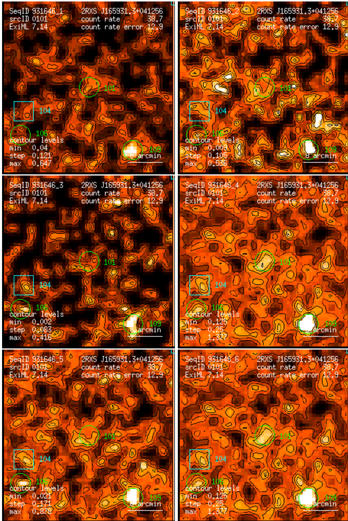
Figure 101: RASS 931646: detection 0101: band rate images, Gaussian filter: (1) PSPC channels 11 – 41, (2) 52 – 90, (3) 91 – 201, (4) 11 – 235, (5) 52 – 201, (6) 11 – 201. Broad band rates in counts/ks. Band rate contour levels in counts/ks/arcmin 2 .
