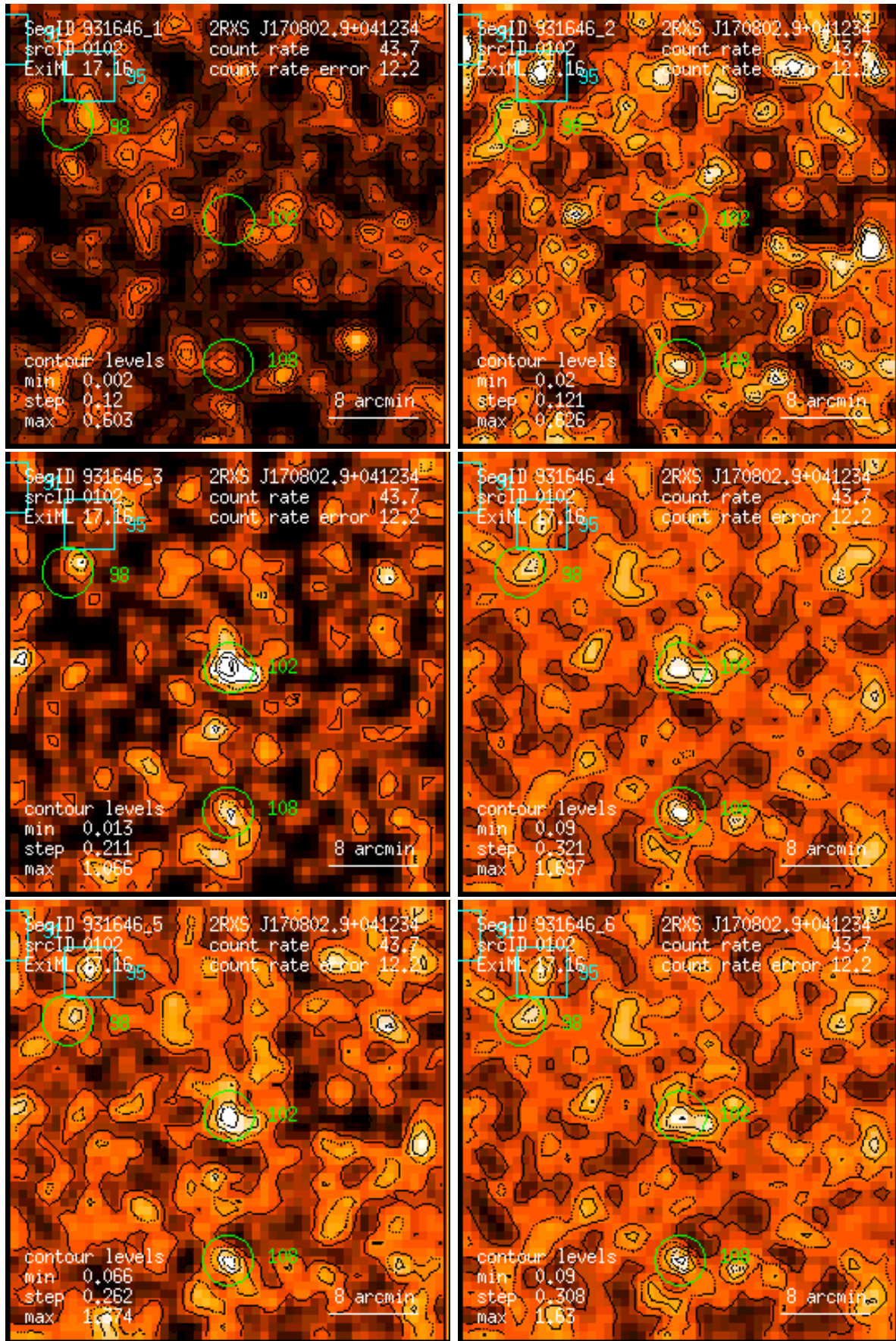
Figure 102: RASS 931646: detection 0102: band rate images, Gaussian filter: (1) PSPC channels 11 – 41, (2) 52 – 90, (3) 91 – 201, (4) 11 – 235, (5) 52 – 201, (6) 11 – 201. Broad band rates in counts/ks. Band rate contour levels in counts/ks/arcmin 2 .
