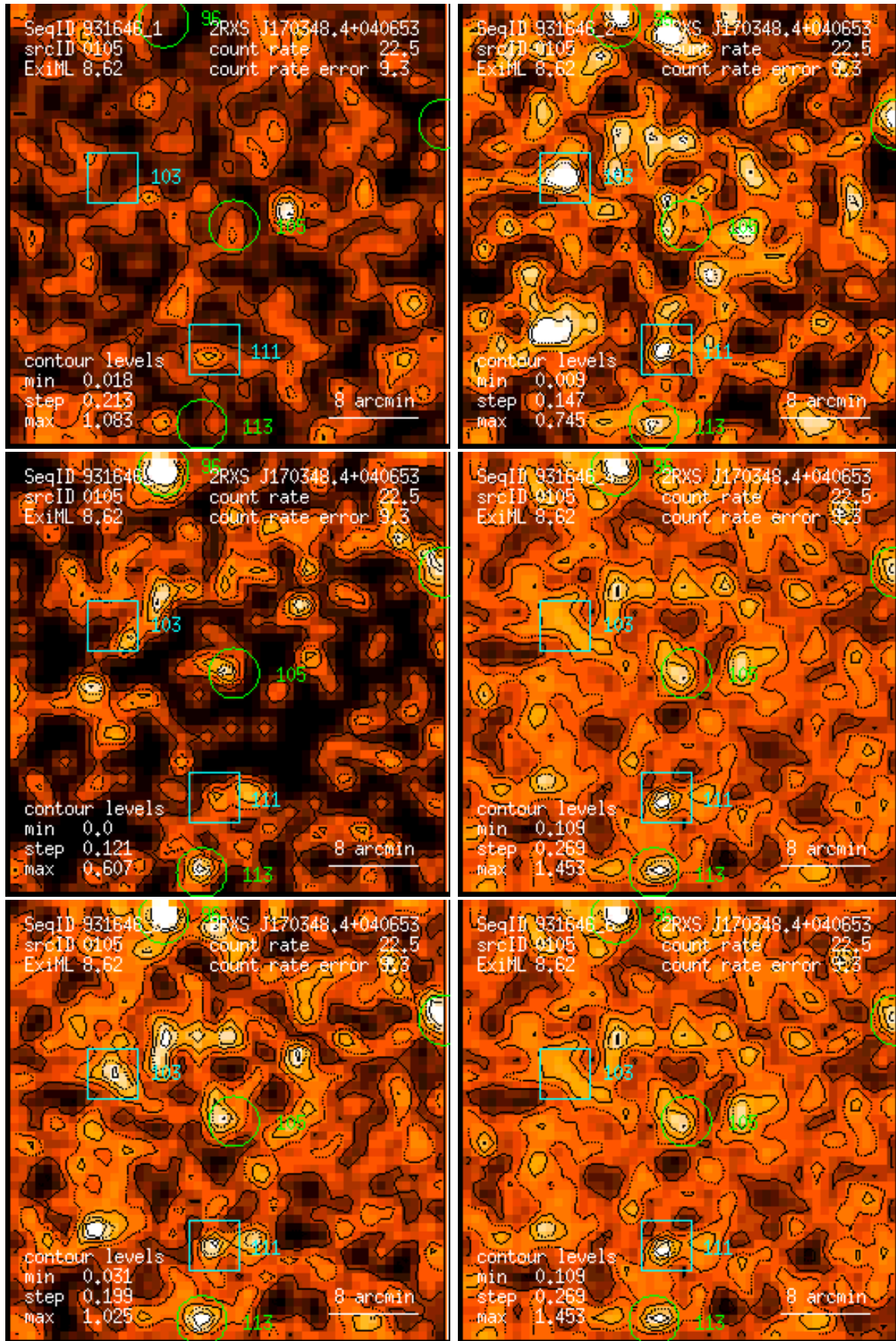
Figure 105: RASS 931646: detection 0105: band rate images, Gaussian filter: (1) PSPC channels 11 – 41, (2) 52 – 90, (3) 91 – 201, (4) 11 – 235, (5) 52 – 201, (6) 11 – 201. Broad band rates in counts/ks. Band rate contour levels in counts/ks/arcmin 2 .
